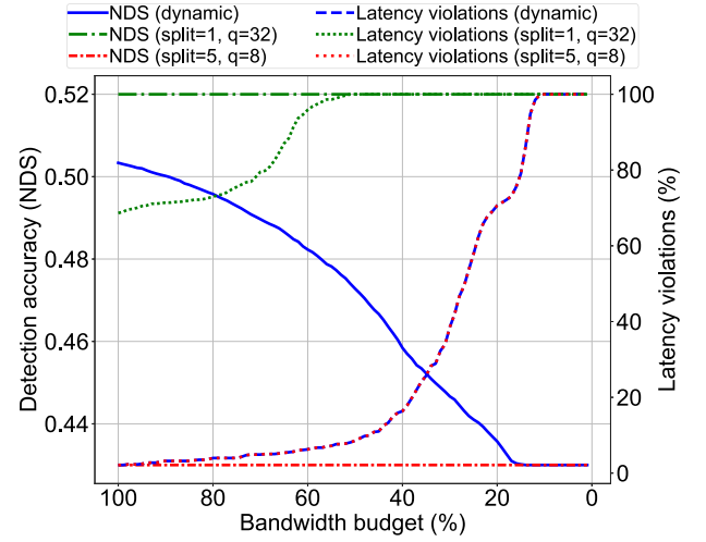
Fig. 10. Detection accuracy (NDS) and number of latency bound violations, as a function of bandwidth dedicated to the perception task, for the dynamic parameter selection algorithm, the highest-accuracy static algorithm ( split = 1 , FP32), and the latency minimizing static algorithm ( split = 5 , FP8).
