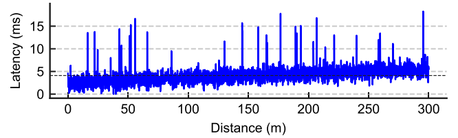
Fig. 3. CPM transmission latency versus distance between a moving vehicle (25 km/h avg.) and a stationary receiver at fixed coordinates (longitude: 6.161993, latitude: 49.626478). Dashed line shows average latency 4.10 ms.
