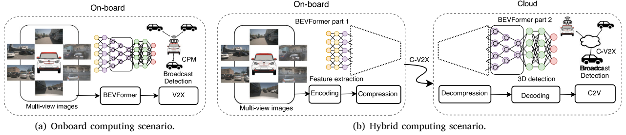
Fig. 1. In the Onboard Computing scenario, the BEVFormer model runs locally, transmitting detection results as CPMs over ITS-G5. In the Hybrid Computing scenario, a compressed feature vector is sent via C-V2X to the cloud for intensive processing, with detection results broadcast to nearby vehicles.
