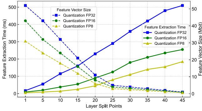
Fig. 4. Feature vector size and extraction time versus split depth. Solid lines represent feature extraction time (left y-axis), while dashed lines indicate feature size (right y-axis). Lower-precision quantization (e.g., FP16, FP8) reduces both extraction time and feature size.
