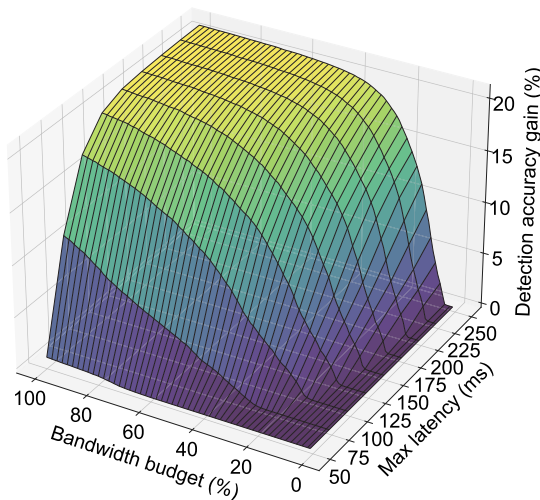
Fig. 11. Detection accuracy (NDS) gain offered by dynamic selection algorithm, as a function of the amount of bandwidth assigned to the perception task.
