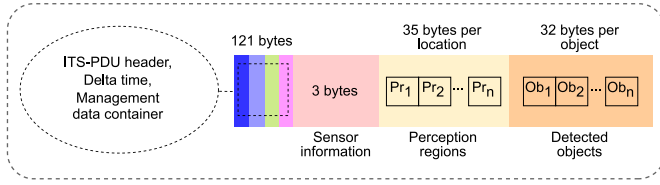
Fig. 2. A basic overview of different containers included in the CPM message format as defined by the ETSI standard [23].
