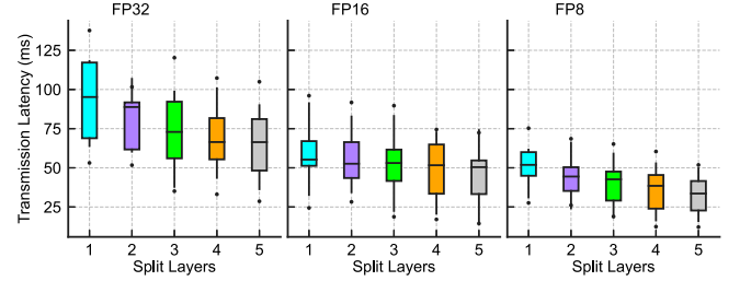
Fig. 5. Transmission latency of feature vectors from vehicle to cloud across five split layers for FP32, FP16, and FP8 over a 5G network using C-V2X. FP8 demonstrates the lowest and most stable latency, suitable for real-time transmission. FP32 exhibits the highest latency and variability, especially at earlier split layers due to larger feature size.
