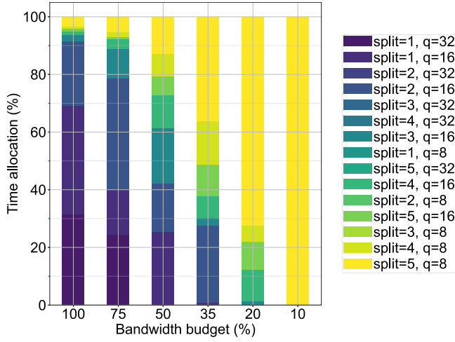
Fig. 9. Distribution of parameter tuple usage by dynamic selection algorithm, as a function of the amount of bandwidth dedicated to the perception task.
