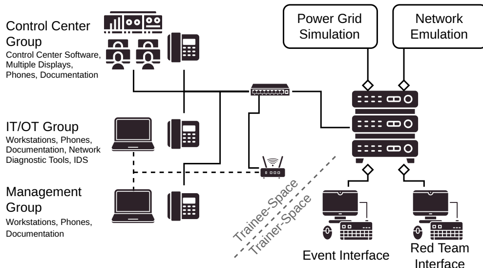
Figure 6: During the training, POWERRANGE combines various physical/real-world interactions for trainees with virtual ones that are conducted by the trainers. While trainees interact with common and specialized software, phones, company procedure guidelines, documentation and external actors (government entities, customers, technicians) represented by trainers via phone or mail, the trainers can implement these actions within the training environment via the event interface, which directly links to the co-simulation environment. Trainers further take the role of the attackers via the red team interface.
