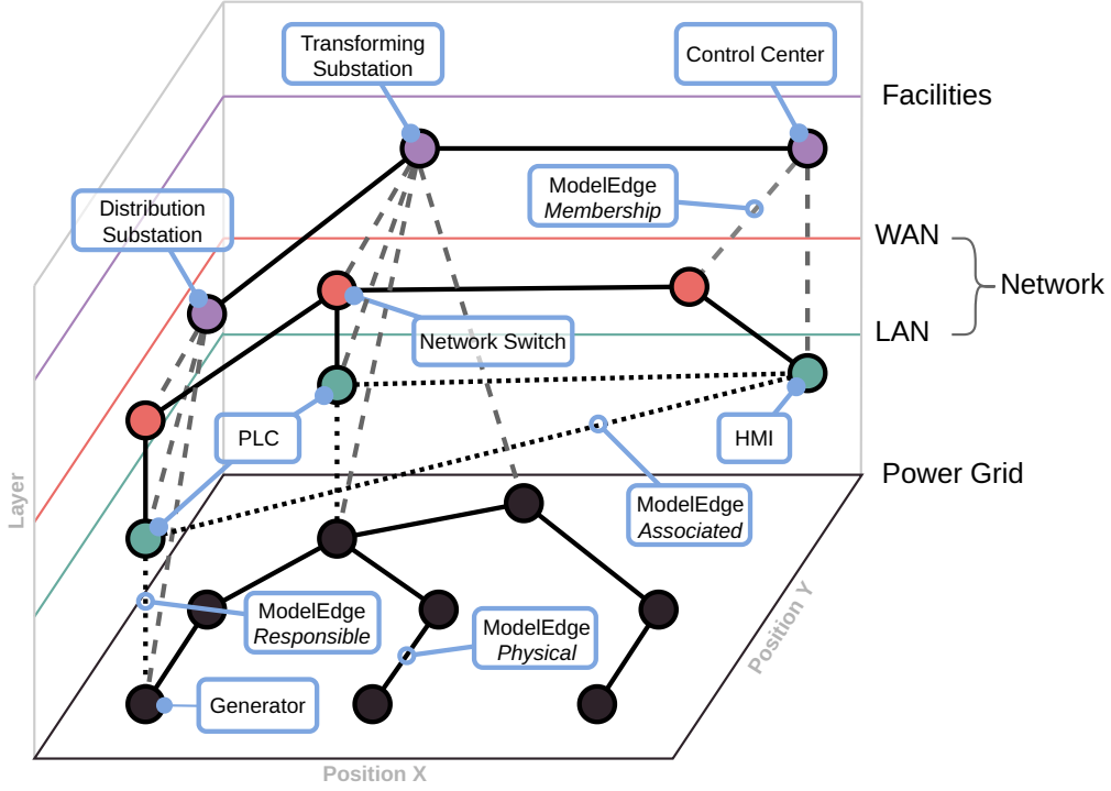
Figure 4: The Multi-Layer Graph (MLG) structures entities, such as power grid and network elements, and facilities on hierarchical layers. Edges between nodes indicate their relationships and interactions. They can cross layer boundaries. The schematic representation of a simplified MLG features three top-level layers, with two sub-layers for the network layer.
