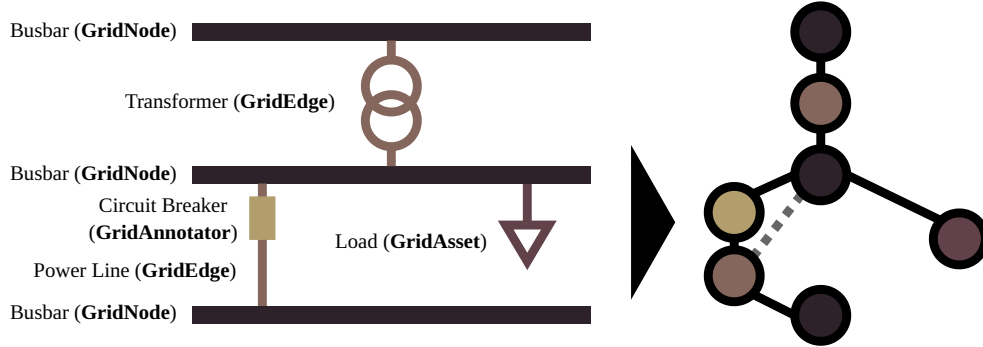
Figure 3: A model of the power grid (left) can be transferred to a graph representation (right), where each grid element is represented by a node and edges represent their, e.g., physical or logical, relations.
