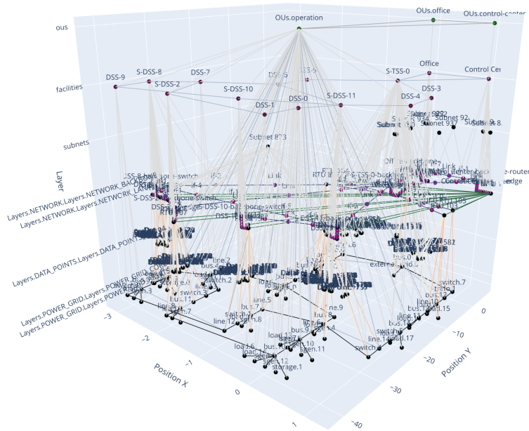
Figure 7: The MLG resulting from a small medium-voltage distribution grid contains entities and their relations from several domains. Besides the power grid itself, resulting facilities such as transforming and distribution substations, a control center, and offices are represented in the graph. Networking equipment, covering hosts and switches, links and individual interfaces are derived based on the facilities and the power grid's topology. Finally, the power grid and network equipment are linked by including OT network protocol configurations, e.g., data point information for the IEC 104 protocol.
