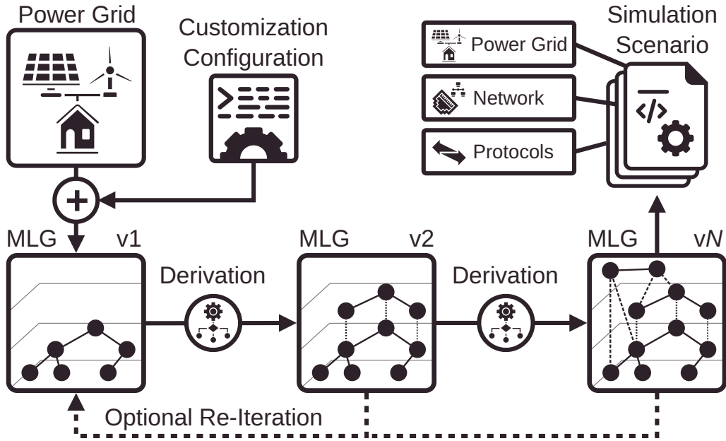
Figure 5: The derivation process follows an iterative approach where multiple Derivators refine the training scenario model based on its MLG representation. Each phase can add, modify or remove information based on the provided customization options, e.g., the desired digitization level. When required, a re-iteration can be initialized to refine earlier derivation phases with contextual information from later stages. Finally, the resulting scenario model can be exported as a ready-to-use simulation scenario.
