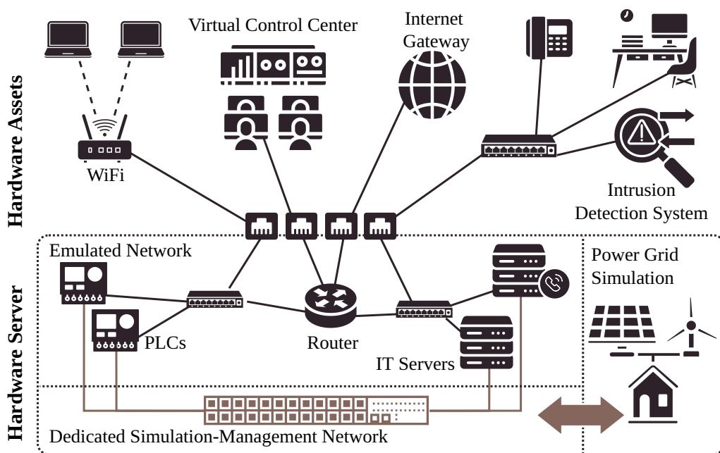
Figure 1: POWERRANGE uses WATTSON to create a digital twin of the power grid and its ICT network. All devices that the participants should interact with can be attached as hardware devices to the emulated network, creating an immersive and realistic training environment.
