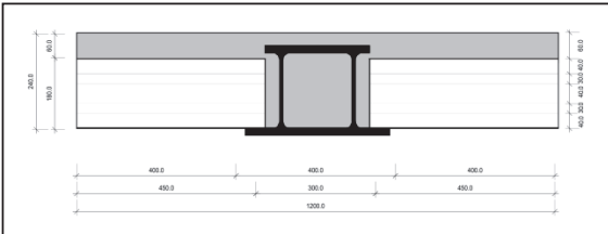
Figure 5: Dimensions of the cross-section of the shallow floor beam
