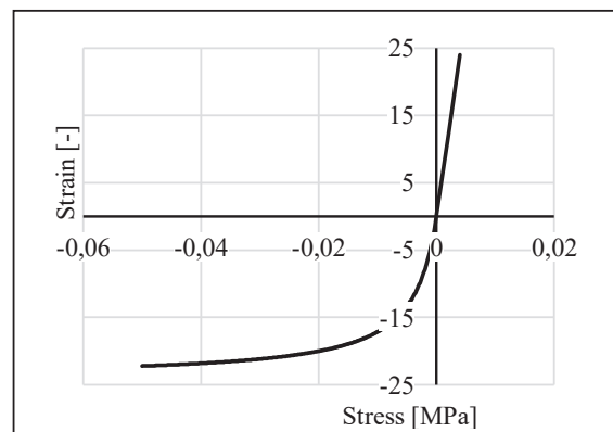
Figure 8: Timber material law for the beam 4C20
