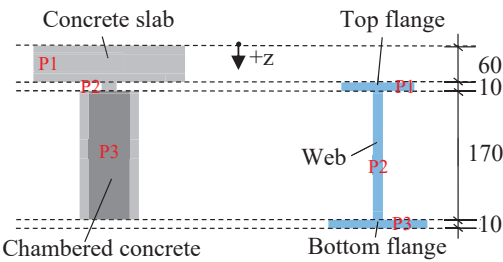
Figure 6: Partitioning of the concrete (left) and steel (right)
