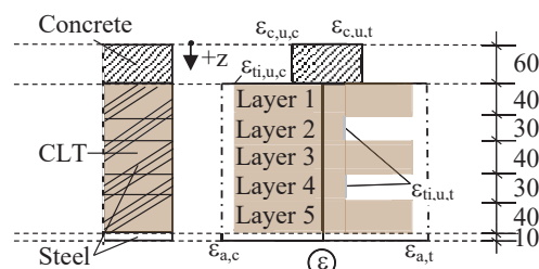
Figure 4: Strain boundaries of the analysed STCC shallow floor beam
