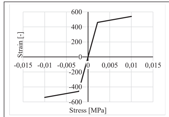
Figure 10: Steel material law for the beam 4C20
