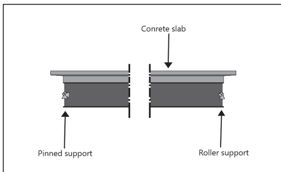
Figure 12: Scheme of the support conditions of a simple composite beam
