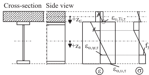
Figure 1: Example of the strain and stress distribution for a composite beam with no shear connection ( \eta=0 )
