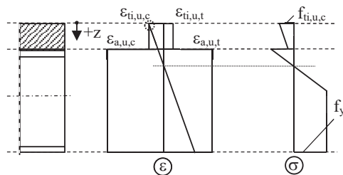
Figure 2: Example of the strain and stress distribution for composite beam with full shear connection ( \eta=1 )
