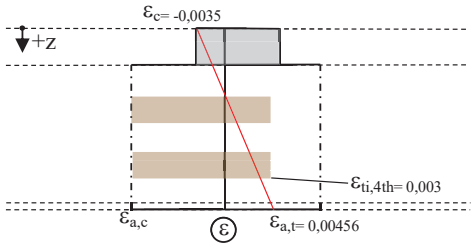
Figure 7: Strain distribution of the 4C20 STCC shallow floor beam
