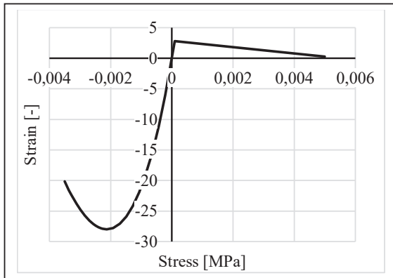
Figure 11: Concrete material law for the beam 4C20
