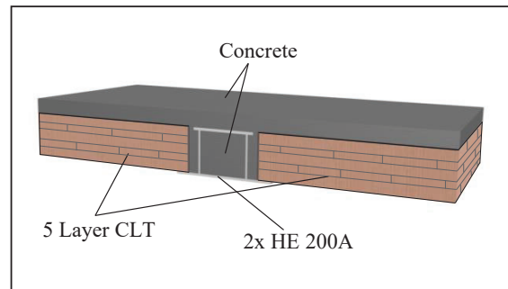
Figure 3: Steel-timber-concrete composite shallow floor beam layout
