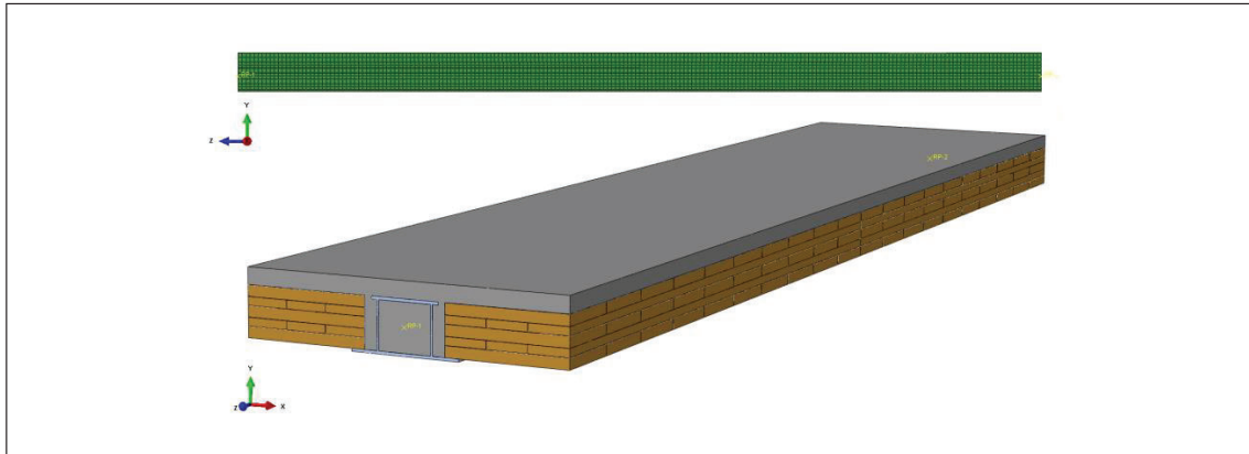
Figure 9. Numerical model of the composite beam in the FE-software Abaqus©, mesh (top), Material visual representation (bottom)
