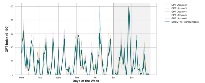
Fig. 4. Representative occupancy pattern for a bus stop using soft DTW barycenter
