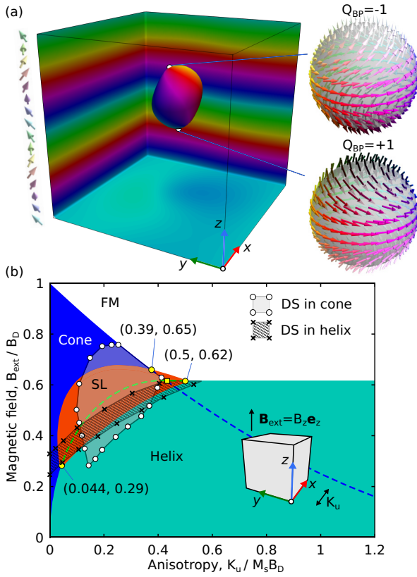
FIG. 1. (a) Stable DS solution in the cone phase obtained by direct energy minimization of Eq. (1) at h = B_{\text{ext}}/B_D = 0.55 and u = K_u/(M_s B_D) = 0.25 , visualized via the isosurface ( n_z = 0 ). The inset highlights two Bloch points (BPs) with opposite topological charges [33]. The standard color code [34,35] is used throughout: white and black pixels indicate magnetic moments aligned parallel and antiparallel to the z axis, respectively, while red, green, and blue represent the azimuthal angle relative to the x axis. (b) State diagram for chiral magnets under an external field applied orthogonally to the hard axis of the magnetocrystalline anisotropy. The red region corresponds to the skyrmion lattice (SL), and the dashed green line marks the conditions where the metastable cone and helix phases have identical energies. The dashed blue line, instead, marks the critical field at which the cone saturates to a FM state. The two semitransparent regions indicate the stability domains of DSs within the cone and helix phases.
