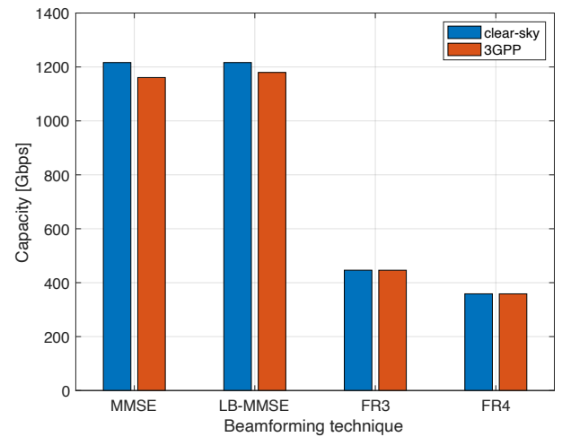
(b) System capacity with user-centric beamforming.
