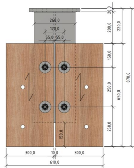
Figure 10: Dimensions of the push-out test specimens.
