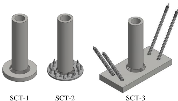
Figure 4: Shear connection devices developed in Prefa-SeTi project.
