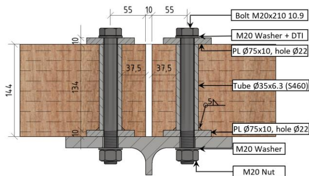
Figure 5: Details of shear connection type 1 (SCT-1).
