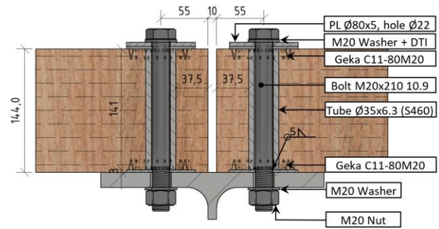
Figure 6: Details of shear connection type 2 (SCT-2).
