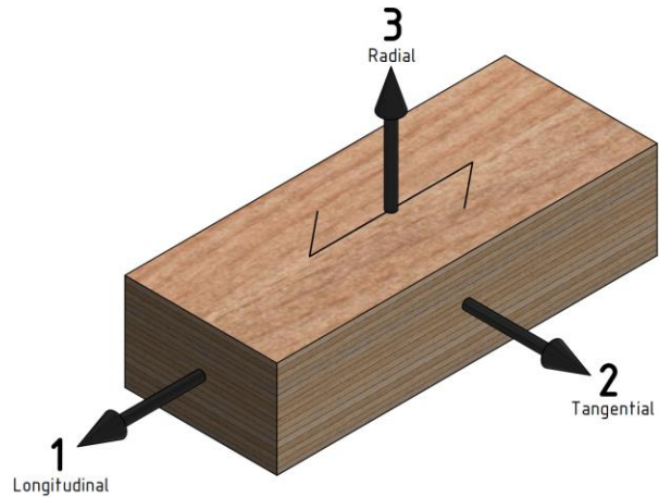
Figure 2: Orthogonal directions of the LVL.
