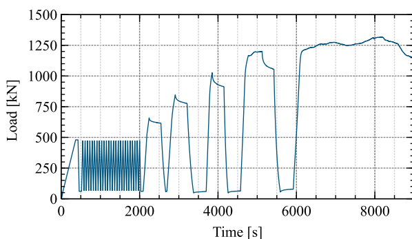
Figure 13: Time history of the loading sequence.
