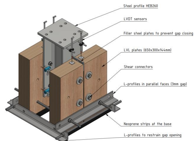
Figure 11: Components of the test setup.
