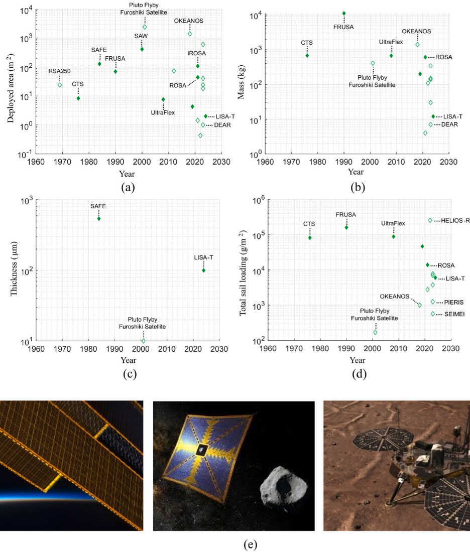
Fig. 17. Solar power sail. Time history, among sails in the database in Appendix B , of: (a) deployed area, (b) mass, (c) thickness, and (d) total sail loading. For flown missions, the year indicates the date of launch. For concepts, the year is the approximate date of first description. Images in (e) are of (left) the Solar Array Wings (SAW) of the ISS, (middle) OKEANOS, and (right) UltraFlex deployed from the Phoenix Mars Lander, with sources in Appendix A .
