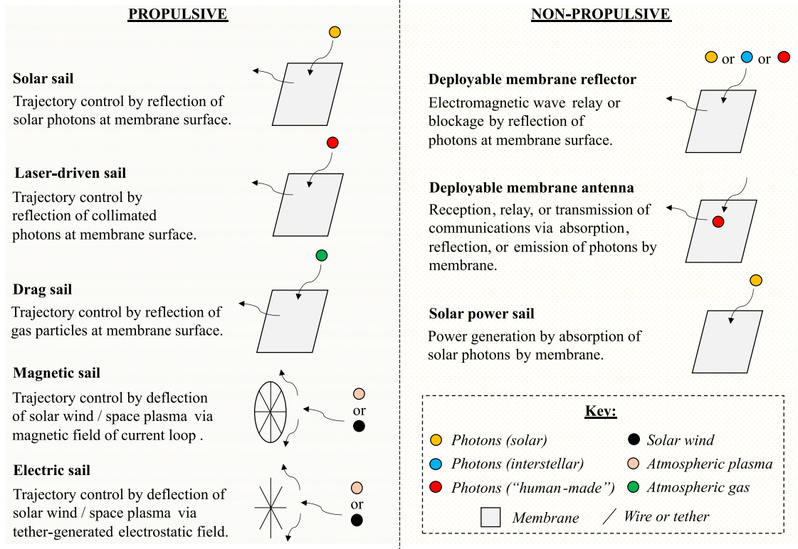
Fig. 5. Spectrum of space sail technologies, divided into propulsive and non-propulsive categories. The basic function of each is indicated. The type of medium needed for the sail to achieve its function is shown. The main structure consists either of one or several membrane(s), or wire(s) and tether(s). Drag sails are categorised as propulsive, in the sense that they provide a delta-V in a planetary atmosphere.
