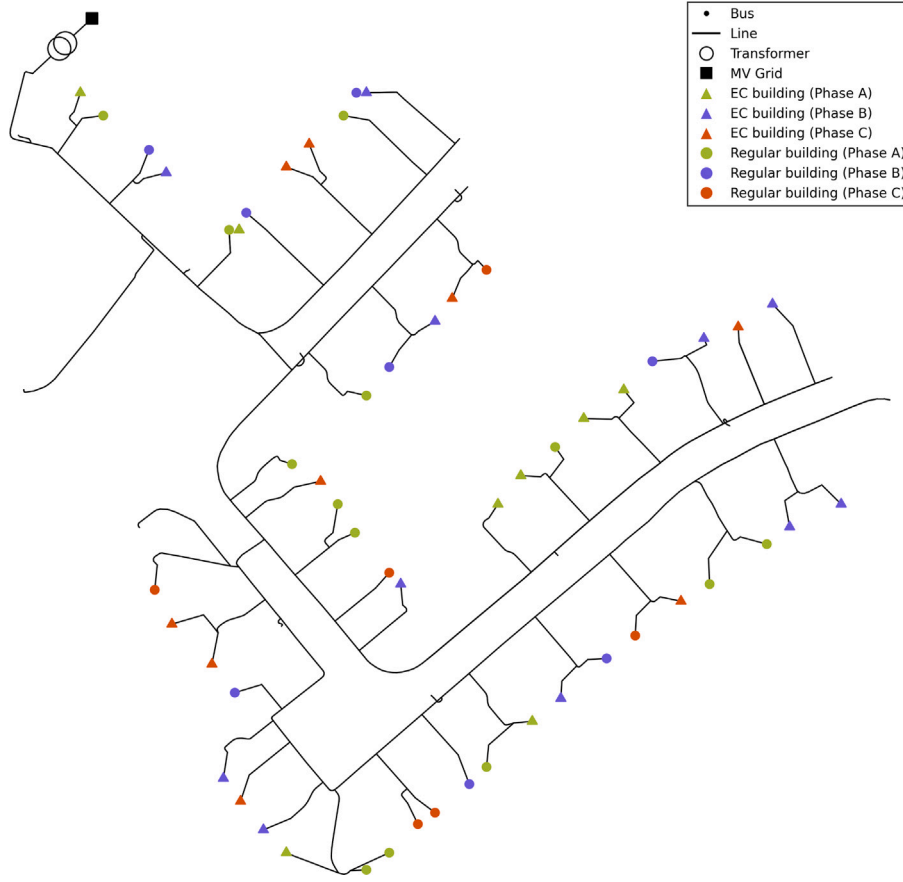
Fig. 2.2. Schematic representation of the studied IEEE European LV DN.
