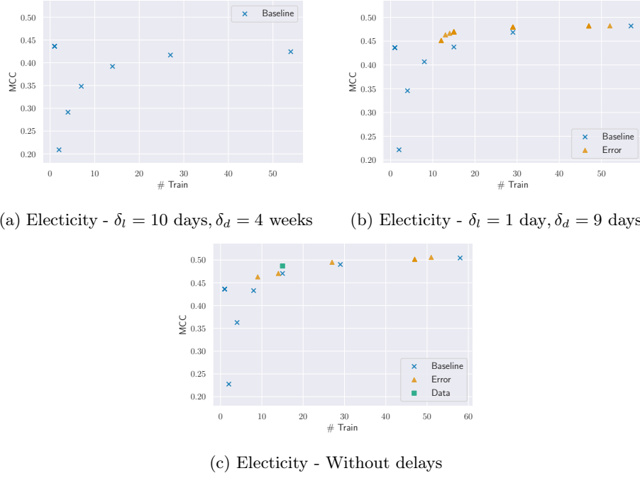
Fig. 4: Pareto front of drift detectors, no retraining and periodic retraining schedules on Electricity dataset.
