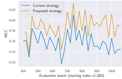
Fig. 1: Evolution of ML effectiveness (MCC) with time (in batches of 20,000 inputs).
