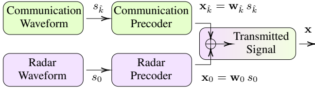
Fig. 3: Beamforming transmission for both communication and sensing.
