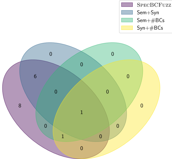
Figure 4: Ablation Study.
