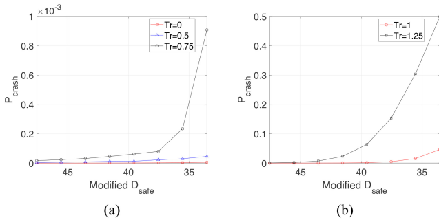
Fig. 6. The probability of having a car crash (collision) for different reaction times versus D_{\text{safe}} which is modified by the worm/attacker. Due to the difference in scales, the curves are divided into two groups; (a) T_r = 0 s, T_r = 0.5 s, and T_r = 0.75 s (b) T_r = 1 s and T_r = 1.25 s. Non-zero T_r values imply that the worm/attacker has disabled hard braking of the ACC module and the driver has reacted after T_r seconds.
