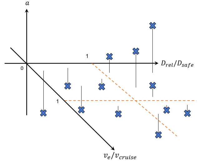
Fig. 7. Three features of the ACC intrusion detection system space along with a few symbolic normal working points. The three features are D_{\text{rel}}/D_{\text{safe}} , v_e/v_c (or v_e/v_{\text{cruise}} ) and a . The fourth one is \tau which could not be demonstrated.
