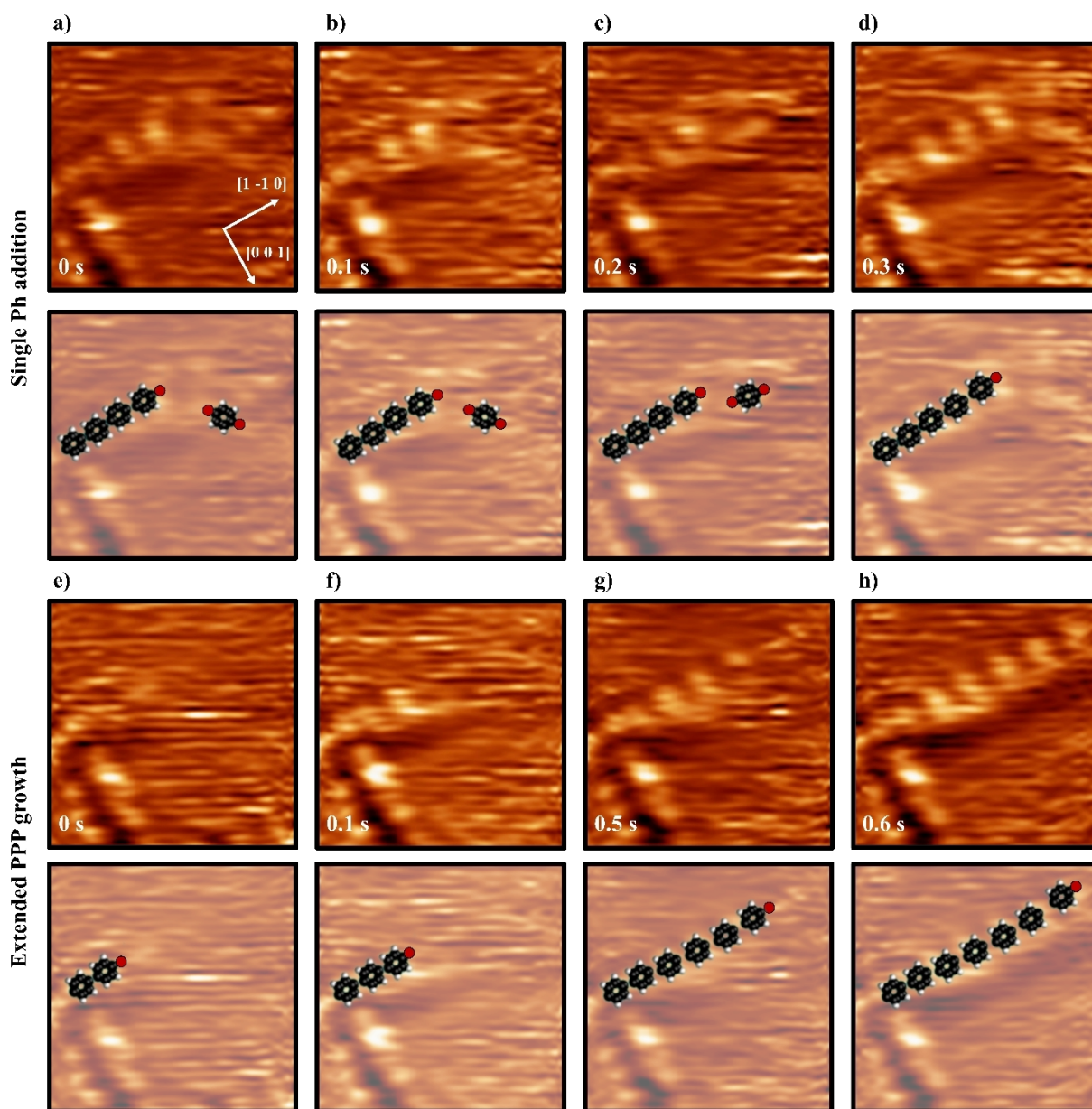
Figure 3. High-speed STM measurements at 150 °C of the growth of PPP chains. a-d) Addition of a single phenylene to a small PPP chain within 300 ms. Red dots are Cu atoms. e-h) Extended growth of a PPP chain. Below each STM image is a schematic of the STM image to visualize
