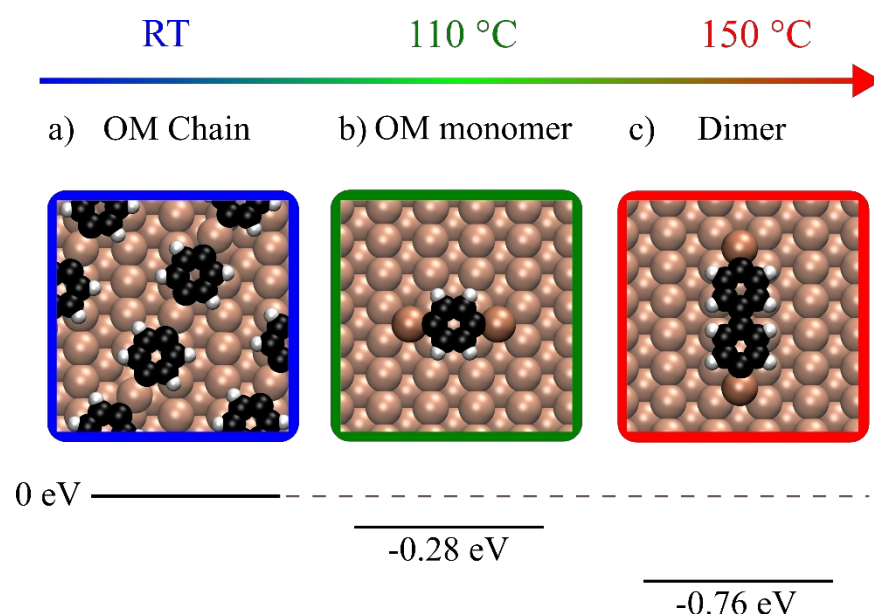
Figure 4. Thermodynamic picture of the stability of different surface species during the temperature evolution. The formation energies for different structures are calculated with respect to the energy of the OM chains observed at RT (-4.69 eV per phenylene). Positive (negative) values refer to less (more) stable structures. Light and dark brown spheres are Cu surface atoms and adatoms, respectively.
