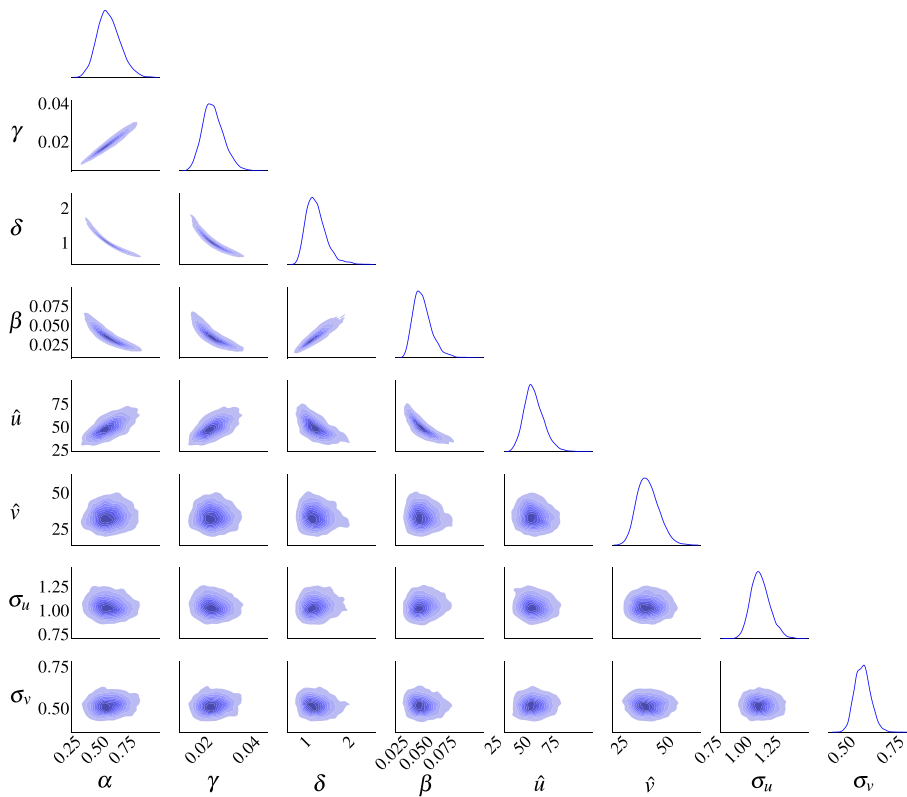
Fig. 1. Plot of posterior distributions associated to p_0 in the Lotka-Volterra model, with posterior marginal distributions on the diagonal and bivariate distributions for outside the diagonal. One can observe high correlations between some pairs of parameters.
