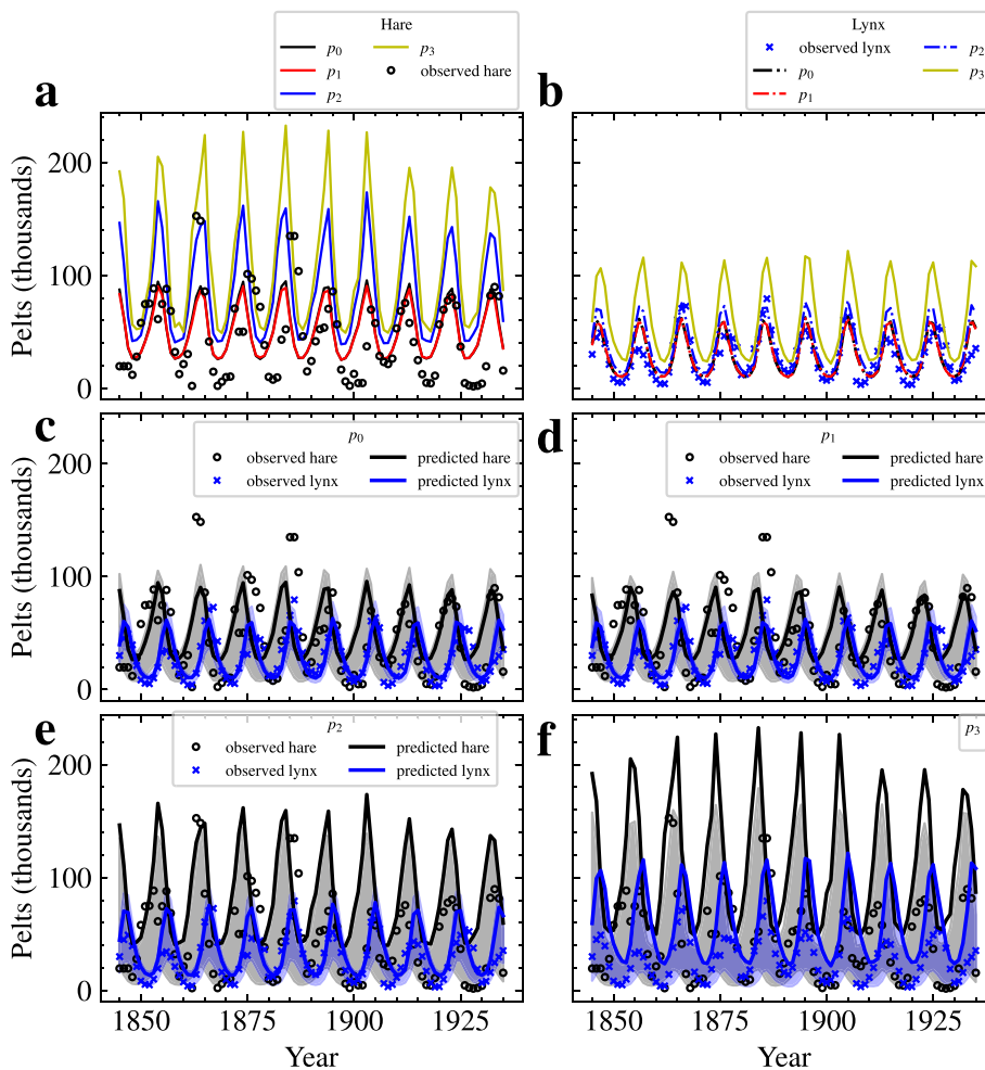
Fig. 2. Graphical posterior predictive check for (a) Hare and (b) Lynx. The prior p_3 has a noticeable visual impact compared to p_0 and p_1 . (c-f) Posterior predictive check for each prior with 25% and 75% quantiles.
