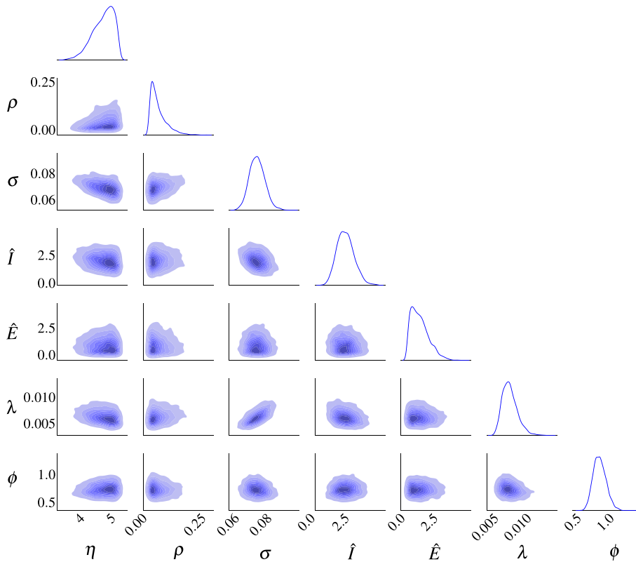
Fig. 3. Plot of posterior distributions associated to p_0 in the SEIR model, with posterior marginal distributions on the diagonal and bivariate distributions for outside the diagonal. There is a high correlation between the parameters \lambda and \sigma .
