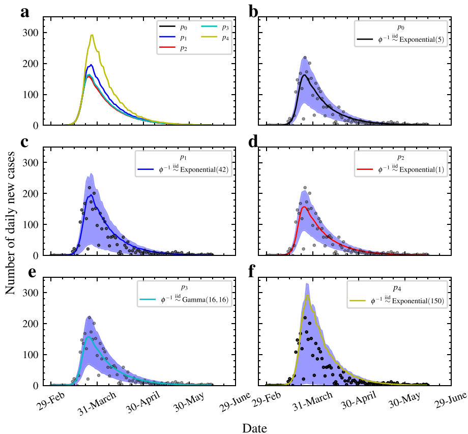
Fig. 4. (a) Graphical posterior predictive check for all priors in the SEIR model, and (b-f) posterior predictive check for each prior with 25% and 75% quantiles. The Gamma(16,16) prior seems to be a better option since the posterior has less variability compared to the other. Moreover, most of the observed counts are in the 25% to 75% prediction bands unlike for other posteriors considered where the highest and lowest counts are outside, or the bands are wider like for Exponential(42). The prior p_4 has the largest predicted values and the predictions are further away from the observed values compared to the other priors.
