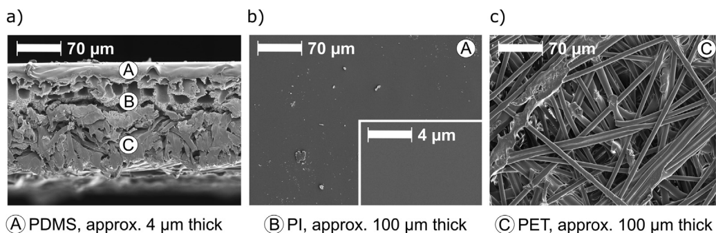
Fig. 4. SEM pictures: (a) membrane cross section, (b) top view of the upper selective PDMS-layer \text{\textcircled{A}} and (c) top view of the lower PET-support layer \text{\textcircled{C}} .
