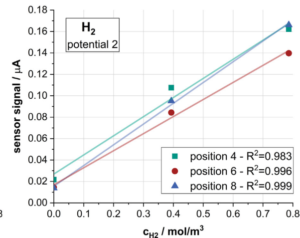
Fig. A2. H_2 calibration curves of the electrochemical sensors mounted in positions 4, 6 and 8 for two different potentials, (a) and (b).
