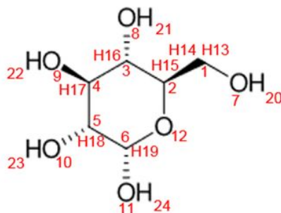
alpha-D-glucopyranose
