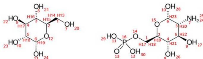
alpha-D-glucopyranose (left)
