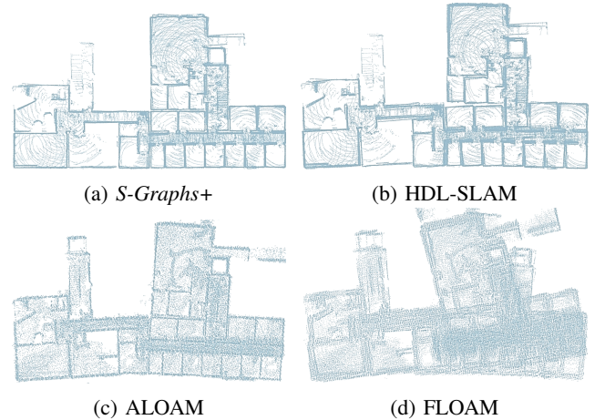
Fig. 3: Maps by S-Graphs+ and baselines, in-house seq. C4F0 .
