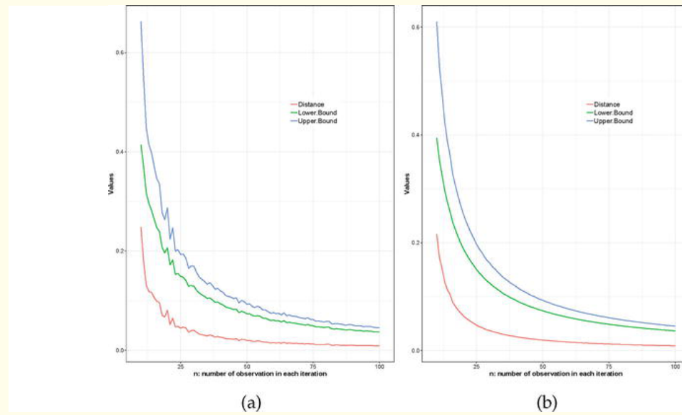
Figure 1. (a) Shows the bounds and the distances between the bounds for N = 100 iterations for each sample size 10–100 by steps of 1, and (b) illustrates the same situation for N = 1000 . The hyperparameters are \kappa = 0.2 and \eta = 2 , while the fixed parameter \alpha equals 0.5.
