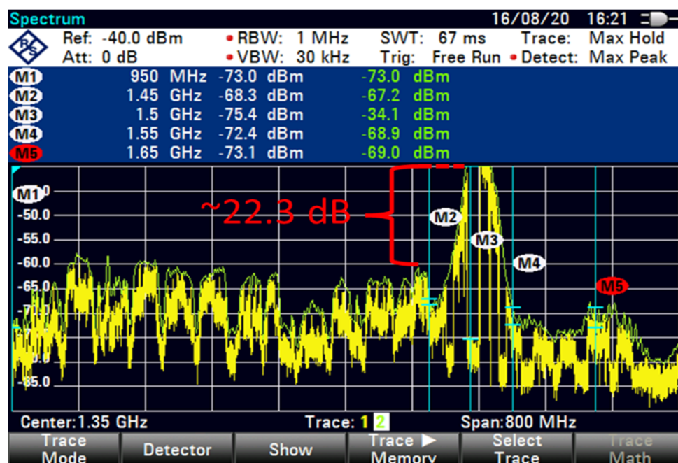
Figure 13. FSS for 85 m (extended C-Band + Filter-1, 50 MHz GB).
