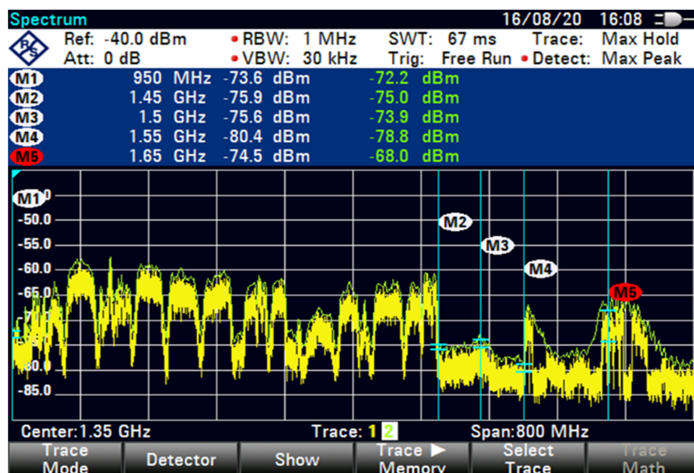
Figure 12. FSS for 85 m (extended C-Band + Filter-1, 100 MHz GB).
