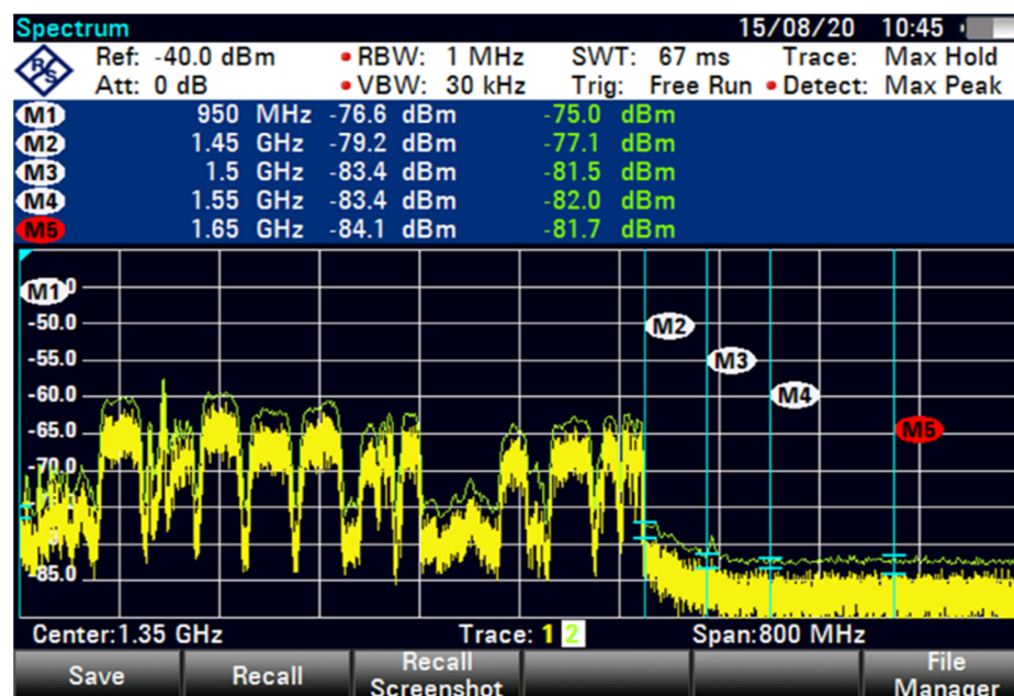
Figure 9. FSS for 85 m (new C-band OFF).
