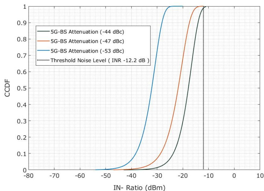
Figure 21. Attenuation CDF for the INR of adjacent interference is based on the out-of-band emission mask of 5G-BS.
