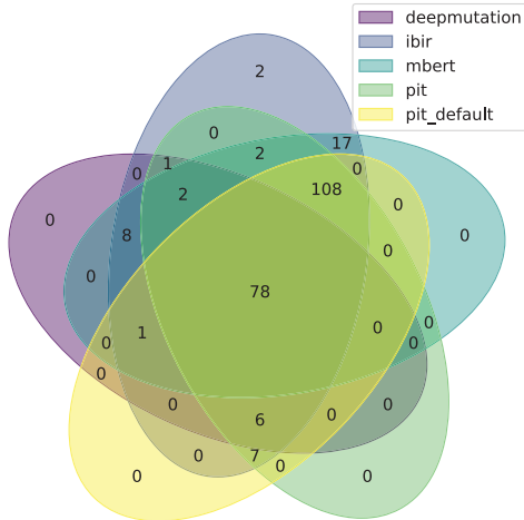
Fig. 3: Which bugs are revealed by every approach? IBIR is capable to find almost all (99,57%) bugs followed by mBERT (92,7%), Pit (87,55%), Pit-default (85,83%) and finally DeepMutation (41,20%).
