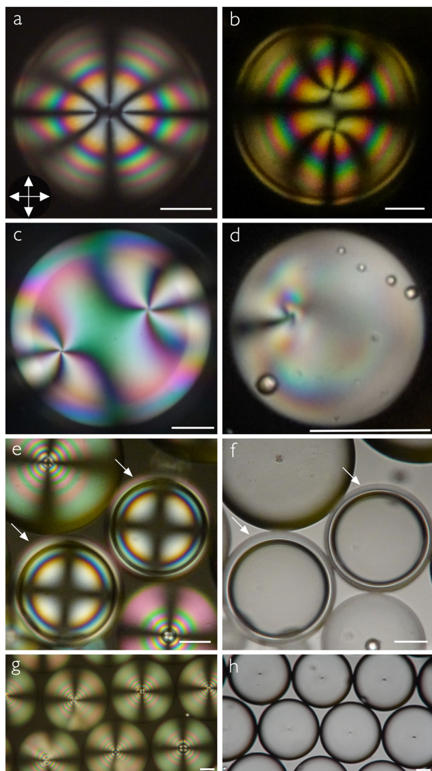
Fig. 2 POM images of shells of (a) MBBA (25 °C), (b) M5N (25 °C) and (c) PCH-5 (45 °C); a droplet of CCH-5 (d); and shells (e), (g) and droplets (f), (h) of MPCC between crossed polarizers (e), (g) and without analyzer (f), (h), at 30 °C. Crossed polarizers are aligned as the double arrows in (a). Scale bar in image (d) represent 50 \mu\text{m} and all other scale bars represent 100 \mu\text{m} .
