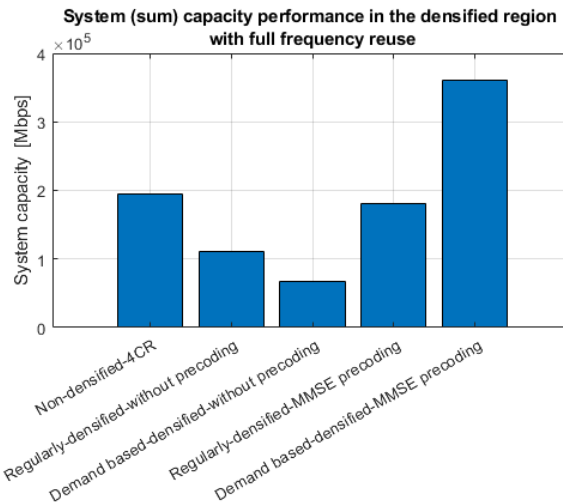
Fig. 26: System (sum) capacity performance based on DVB-S2X at densified area for full frequency reuse
