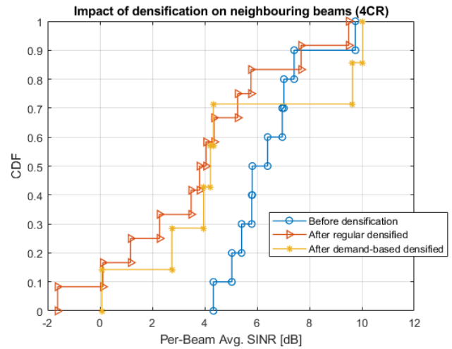
Fig. 38: CDF plots of per beam avg SNIR on neighbouring beams
