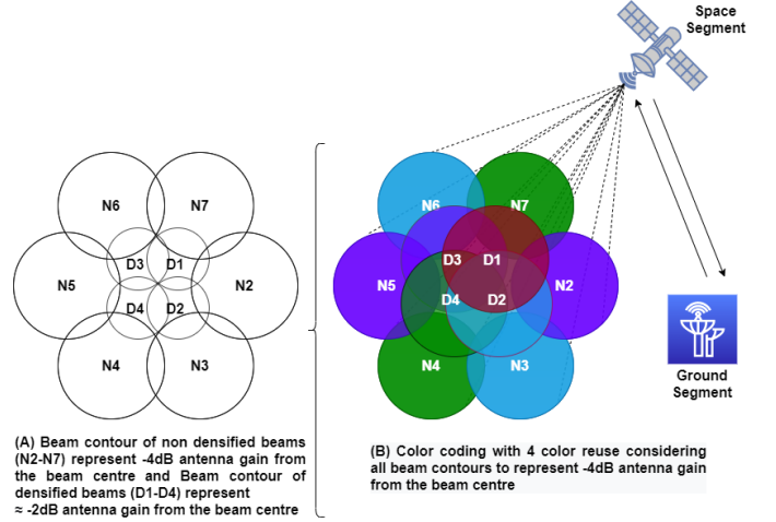
Fig. 3: Regular Beam Densification in the high demand region by replacing one beam with four beams increases inter-beam interference.
