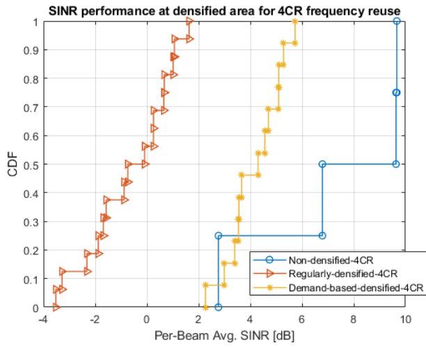
Fig. 16: SINR performance at densified area for 4CR frequency reuse
