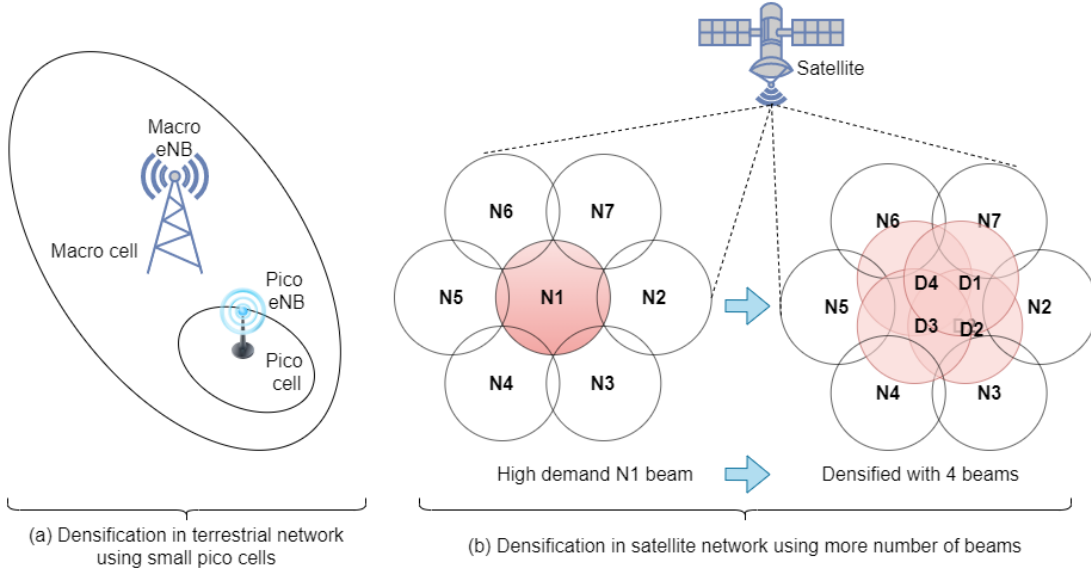
Fig. 2: Beam densification in terrestrial network and satellite network
