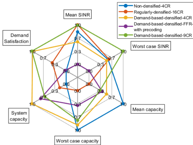
Fig. 40: Radar chart summarising the results
