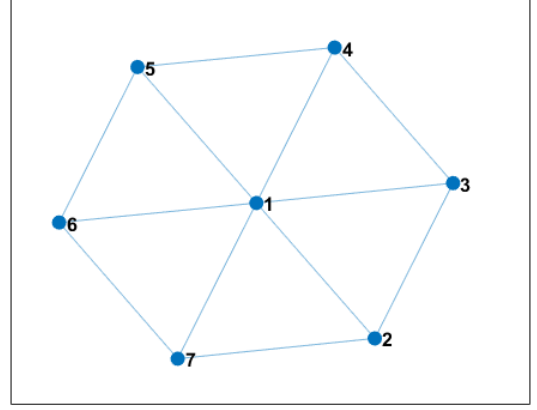
Fig. 11: Graph obtained from the adjacency matrix to the beams in Figure 1.
