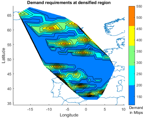
Fig. 7: Uneven demand distribution at the densified region
