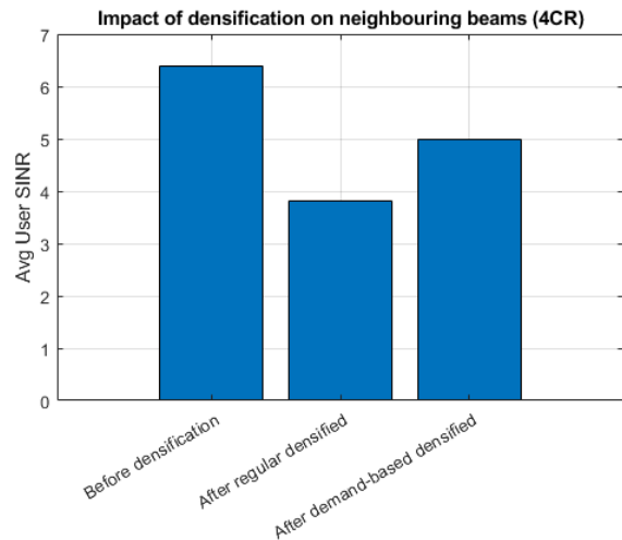
Fig. 39: Average user SINR on neighbouring beams
