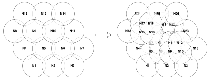
Fig. 9: Non densified 14 beams to the left and densified 26 beams to the right
