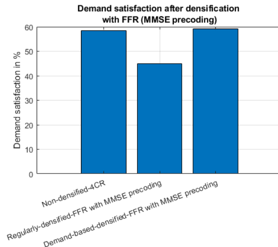
Fig. 27: Demand satisfaction with full frequency reuse
