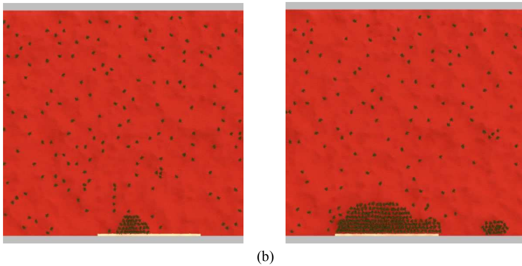
Figure 12: Comparison of different resolution of particles, for flow velocity 500 \mu\text{m/s} : (a) coarse particle distribution; (b) fine particles distribution
