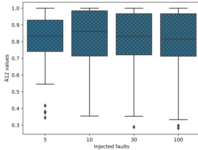
Fig. 11. Vargha and Delaney values for IBiR. \hat{A}_{12} values computed on the detection ratios of injected faults of the test suites that detect and do not detect the (real) faults.
