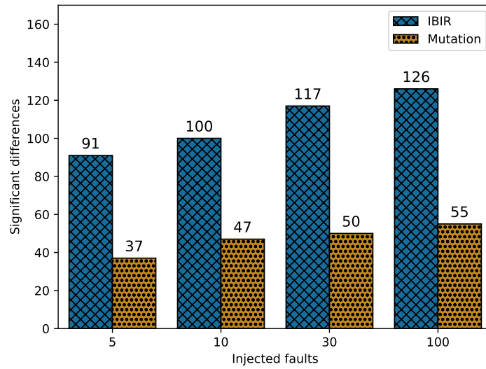
Fig. 10. Number of (real) faults where injected faults provided good indications of fault detection. Particularly, number of cases with statistically significant difference, in terms of ratios of injected faults detected, between failing and passing test suites (wrt real faults).
