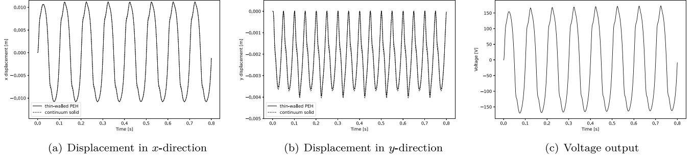
Fig. 14. Displacement of point A and voltage output of the cross-flow-driven PEH.
