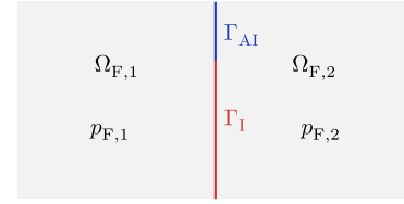
Fig. 3. Splitting domain method to account for pressure discontinuity.
