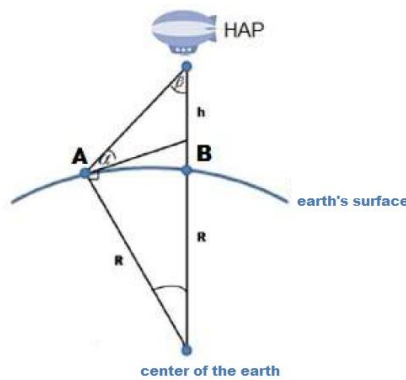
Figure 4. HAP coverage calculation parameters.
