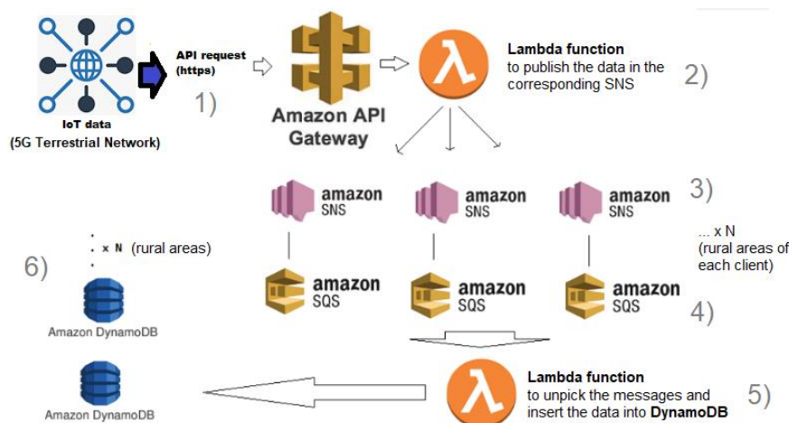
Figure 9. AWS architecture of the smart rural system.
