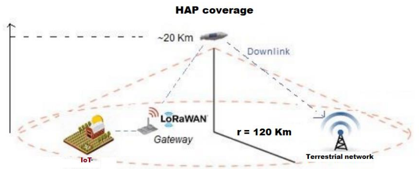
Figure 5. HAP coverage at 20 km altitude
