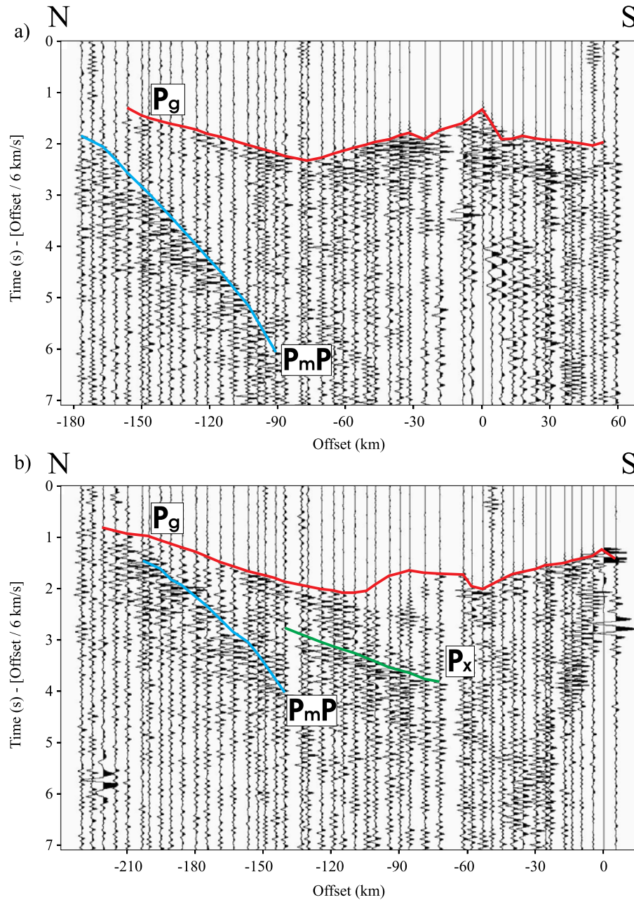
Figure 2. Examples of data recorded by land receivers from land shots. (top) Shot X10. The refracted P waves ( P_g ) are marked in red, and Moho reflections ( P_mP ) are in blue. (bottom) Shot X13. Phases reflected off the “floating” crustal reflector ( P_x ) are marked in green. Reduced traveltimes are shown with a reduction velocity of 6 km/s.
