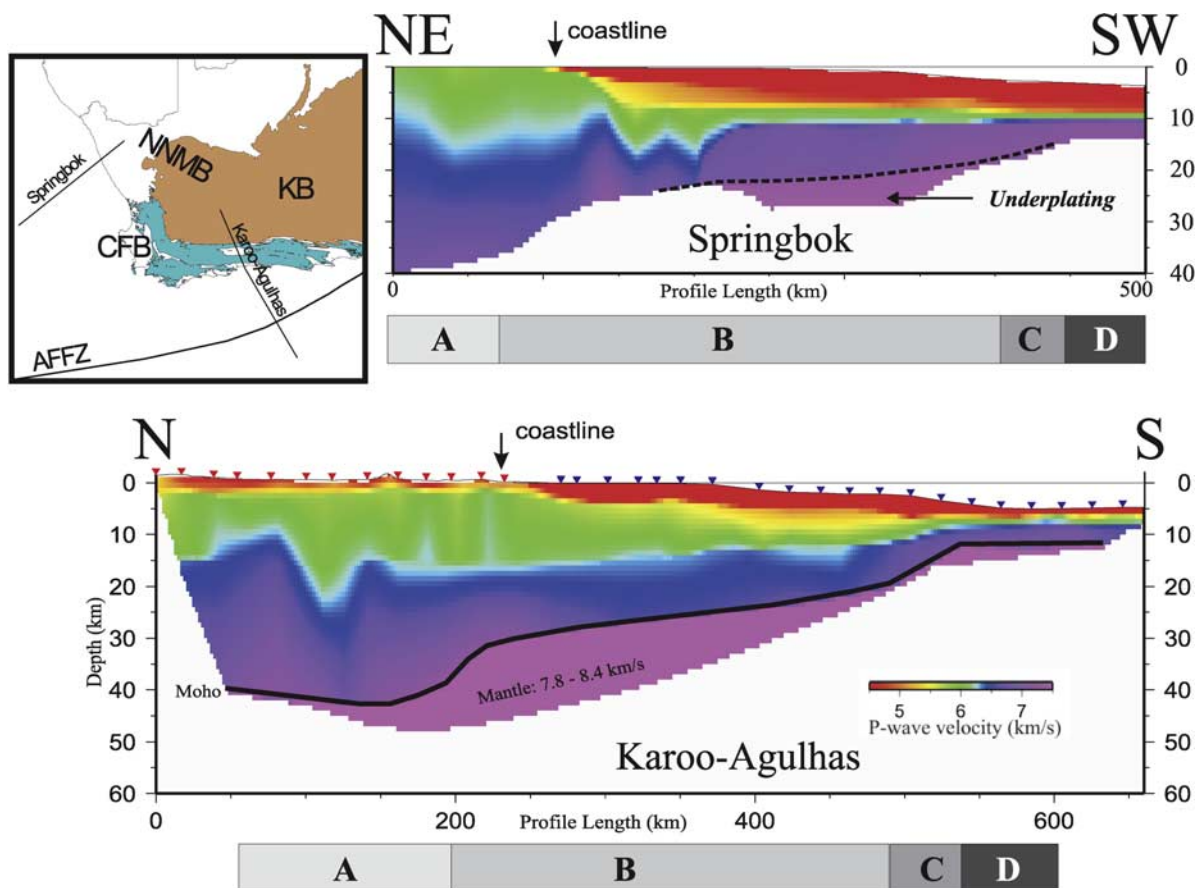
Figure 11. P-wave velocity model comparison between (top) the Springbok profile on the western coast of South Africa [after Hirsch et al. 2008] and (bottom) this study. On the basis of Moho geometry, four segments of the crust can be distinguished in both profiles: (A) thick continental, (B) stretched gradually thinning, (C) steeply thinning, and (D) thin oceanic crust.
