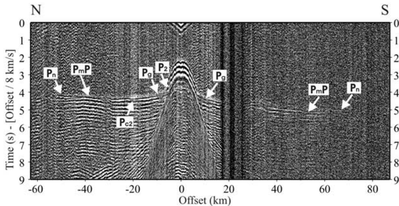
Figure 4. Airgun shots recorded by OBS 105. Phases P_g , P_n , and P_mP are as in Figure 3. P_2 corresponds to P waves refracted in the upper crust low-velocity sediments, and P_{c2} P waves are reflected inside the crust (notation from Parsieglia et al. [2007]). Reduced traveltimes are shown with a reduction velocity of 8 km/s.
