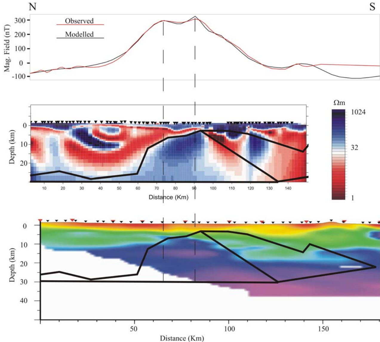
Figure 10. (top) Surface magnetic field (red line) along the profile, compared to the modeled magnetic signature of two magnetic bodies intersected by a few 100 m wide nonmagnetic region [Weckmann et al. , 2007b]. (middle) The two magnetic bodies drawn over the MT depth section of Weckmann et al. [2007a]. (bottom) The magnetic bodies drawn over the northern 180 km of the P-wave velocity model shown in Figure 5. Vertical dashed lines across all three figures project the locations of the maxima of the BMA onto the depth sections.
