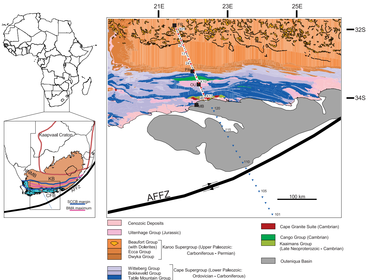
Figure 1. Study area: map of southern Africa showing the relevant large-scale features, like the Kaapvaal Craton, Karoo Basin (KB), Cape Fold Belt (CFB), the location of the Namaqua Natal Mobile Belt (NNMB), the Agulhas-Falkland Fracture Zone (AFFZ), as well the Southern Cape Conductivity Belt and the Beattie magnetic anomaly. The detailed map shows the geological setting of the study area. The onshore section of the profile is indicated by the red triangles (13 shots, numbered X01–X13) and smaller black triangles (48 receivers, numbered 01–48). Four cities are shown on the map to aid the location: Fraserburg (FR), Prince Albert (PA), Oudtshoorn (OU), and Mossel Bay (MB). The 20 ocean bottom seismometers used in the offshore part are marked as blue triangles and are numbered 101–120 following the notation of Parsiegla et al. [2007].
