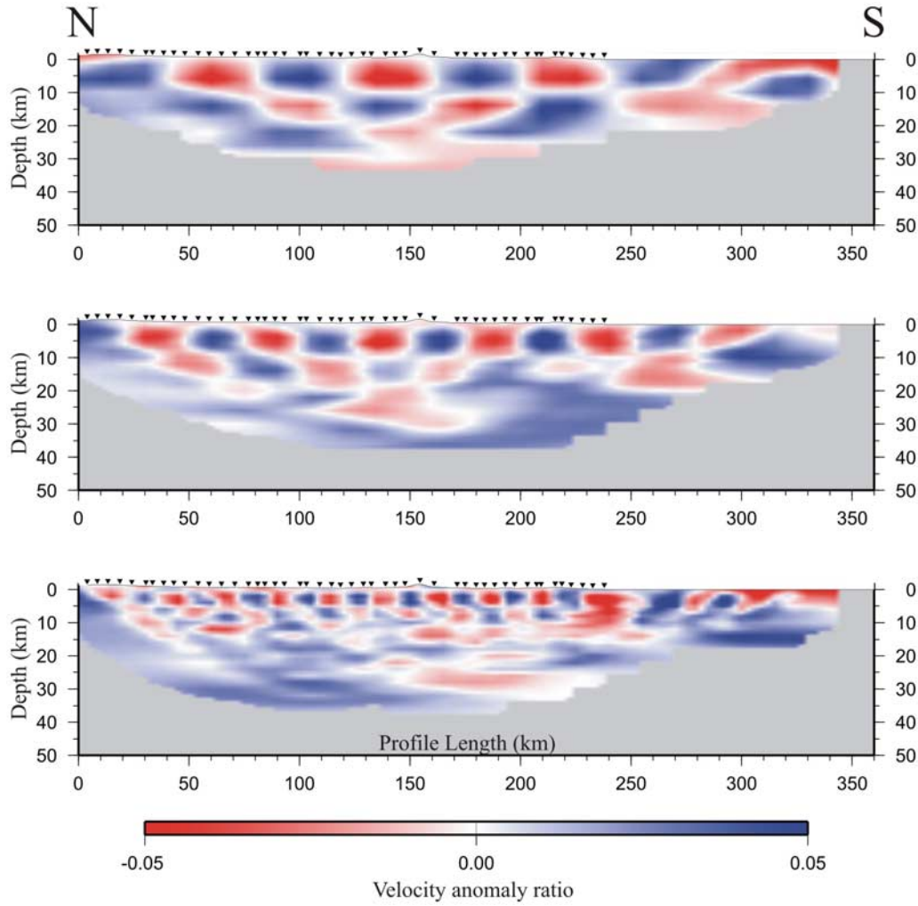
Figure 6. Resolution tests for the model in Figure 5. Original checkerboard sizes are (top) 40 \times 10 km, (middle) 25 \times 10 km, and (bottom) 12 \times 5 km; velocity perturbation of 5% is used in each case.
