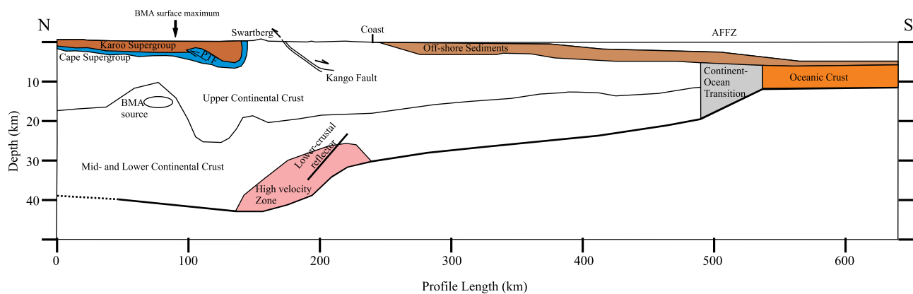
Figure 12. The combined onshore/offshore profile, showing the summary of the findings of this study. To the north the Karoo and Cape supergroups taper out in an asymmetric syncline. The division between upper and middle/lower crust roughly follows the P-wave velocity of 6.5 km/s contour. Near its most shallow point, the high-velocity anomaly most likely related to the BMA is found in the middle crust. Immediately south a large synclinal feature was identified in the upper crust. In the lower crust, high-velocity material has been observed on top of the steeply rising Moho, as was a reflector roughly parallel to the Moho. Offshore the layer of sediments can be seen, as is the structure of the AFFZ, which separates the continental from oceanic crust.
