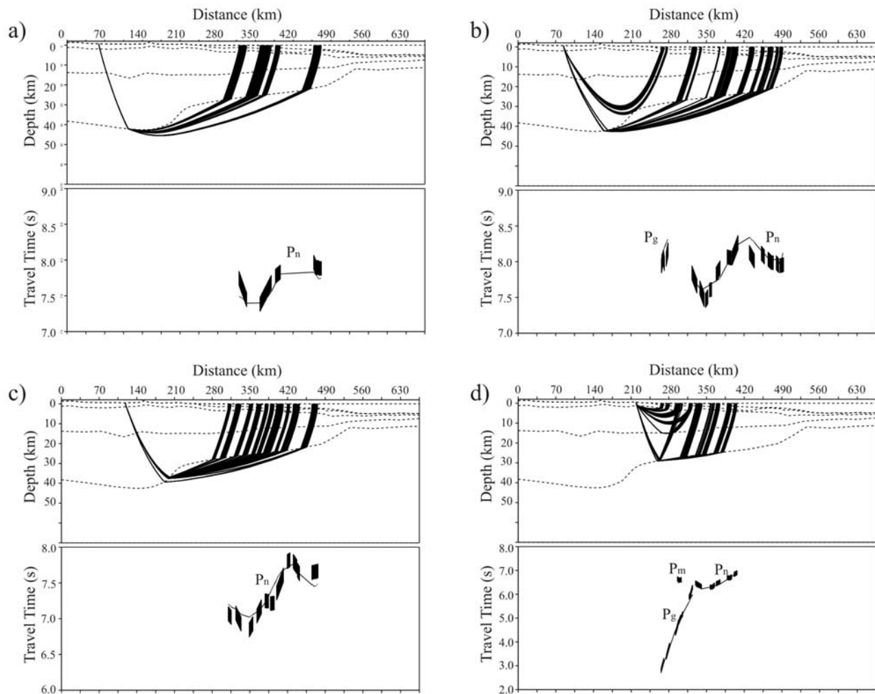
Figure 8. Airgun shots recorded by 4 land receivers: (a) receiver 12; (b) 17; (c) 24; (d) 44. (top) The raypaths; (bottom) the observed traveltimes (steeples corresponding to uncertainty bars) and the traveltimes expected from the model for the given source-receiver distance (solid line).
