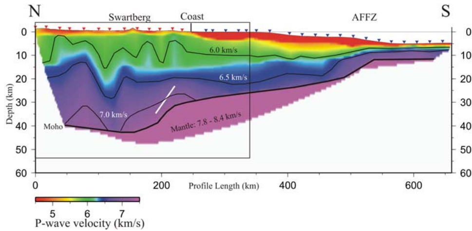
Figure 7. P-wave velocity model for the entire profile. To help the location with Figure 1, land shots (red triangles) and OBSs (blue triangles) have been indicated. Velocity contours corresponding to 6.0, 6.5, and 7.0 km/s have been drawn. The thick white line marks the “floating” reflector. The black rectangle indicates the northern 340 km that is shown in Figures 5 and 6.
