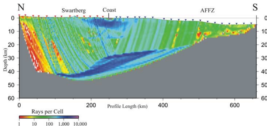
Figure 9. Ray coverage for the model presented in Figure 7. A logarithmic scale of number of rays crossing each 2 km by 1 km cell highlights regions of relatively high or low coverage.
