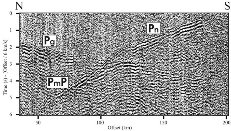
Figure 3. Example of the data from airgun shots picked up by land receiver 46. Direct P waves from the crust ( P_g ), from the mantle ( P_n ), and Moho reflections ( P_mP ) are clearly visible. Reduced traveltimes are shown with a reduction velocity of 6 km/s.
