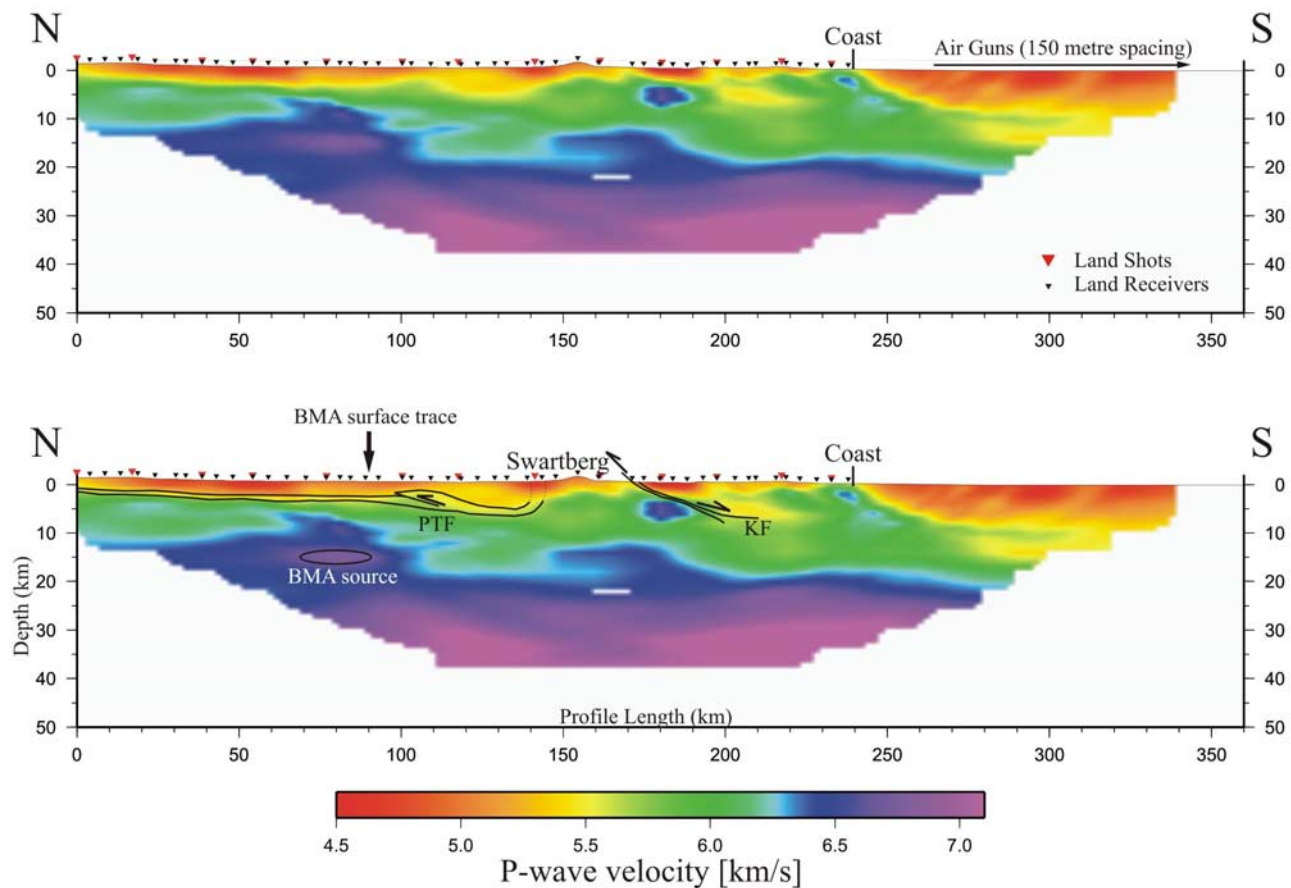
Figure 5. P-wave velocity model computed for the onshore part of the profile, as well as the first 100 km of the offshore part. The top shows just the model, the bottom includes interpretations. Starting in the north, 140 km of the inferred distribution of the Karoo Supergroup, and the Cape Supergroup underlying it, has been drawn. The location of the blind thrust fault, which we believe marks the northernmost deformation of the Cape Supergroup, has been marked by an arrow (PTF). We see the thickening of the basement at profile km 130, which is consistent with the syncline at which it tapers out. The actual edge of it, however, is not resolved and has been drawn in dotted lines. Farther south, the geometry of the normal listric Kango Fault (KF, surfacing at 170 km) has been drawn. A high-velocity anomaly most likely related to the BMA has been indicated with an ellipse at a depth of \sim 15 km, at profile km 80. The center of the surface trace of the BMA has also been indicated.
