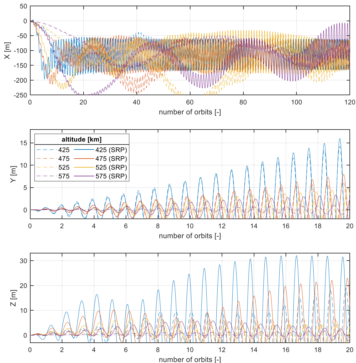
Fig. 14 Formation deployment with eclipse, results for satellite 2
