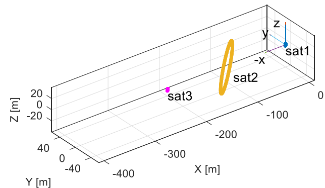
Fig. 12 Target formation geometry
