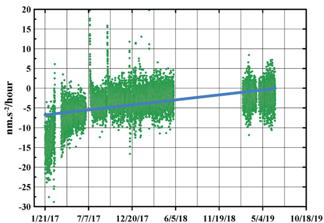
Fig. 5 B Instrumental drift rate of the CG6-003 from different occupations in the WULG
