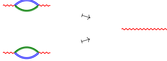
FIGURE 10. 2-to-1 map between colorings of \Gamma and of \Gamma' of Proposition 4.3.
