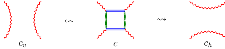
FIGURE 15. Coloring c of \Gamma induces coloring c_v of \Gamma^v and coloring c_h of \Gamma^h .
