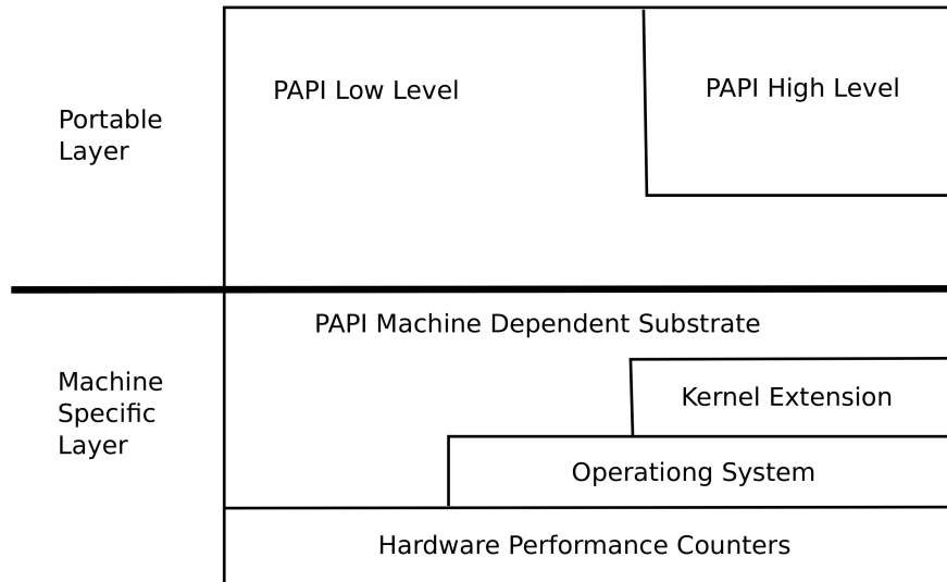
Figure 33. PAPI architecture
