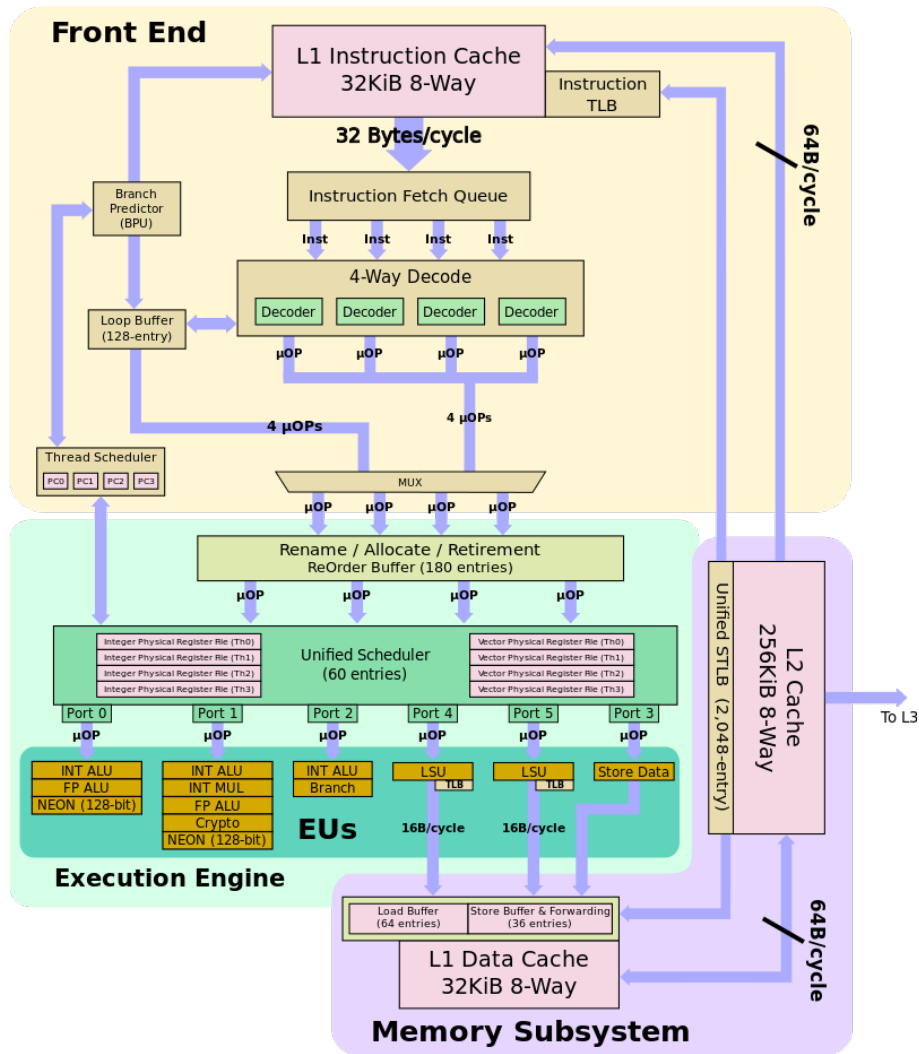
Figure 3. ThunderX2 block diagram [53]
