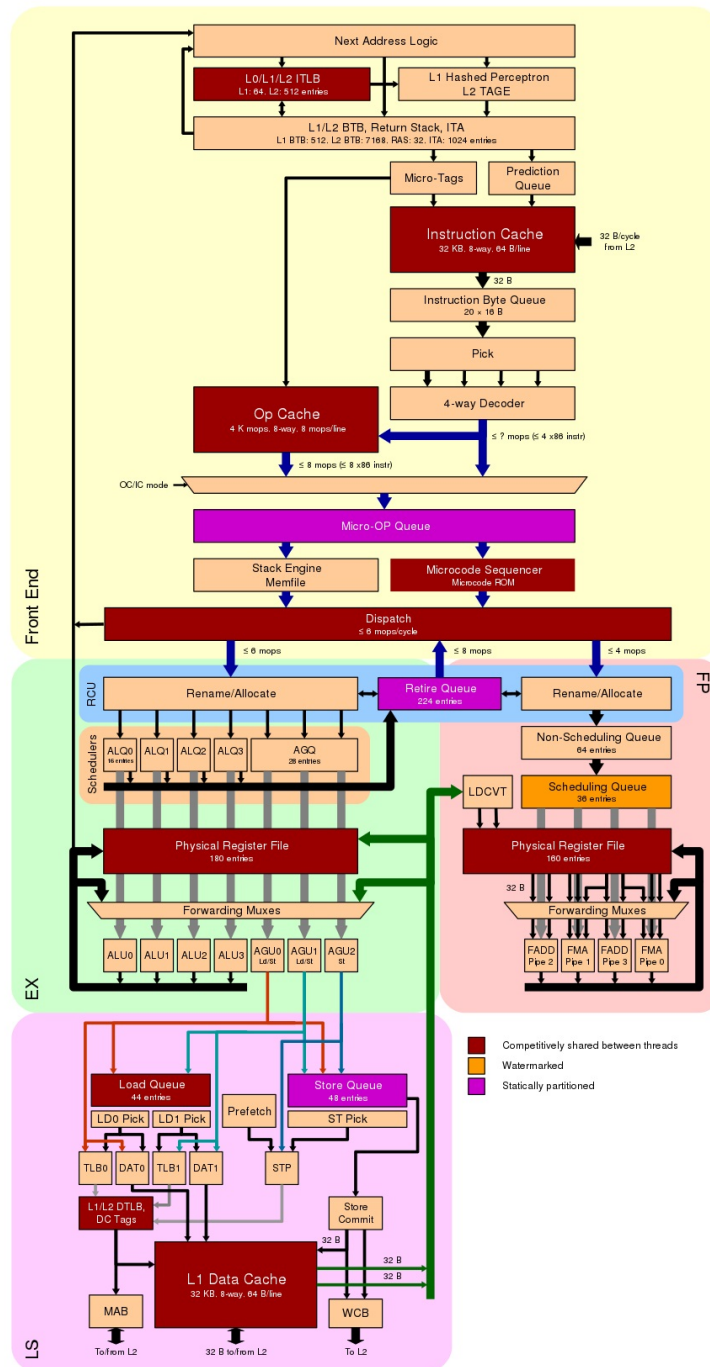
Figure 56. AMD Zen 2 core diagram [44]
