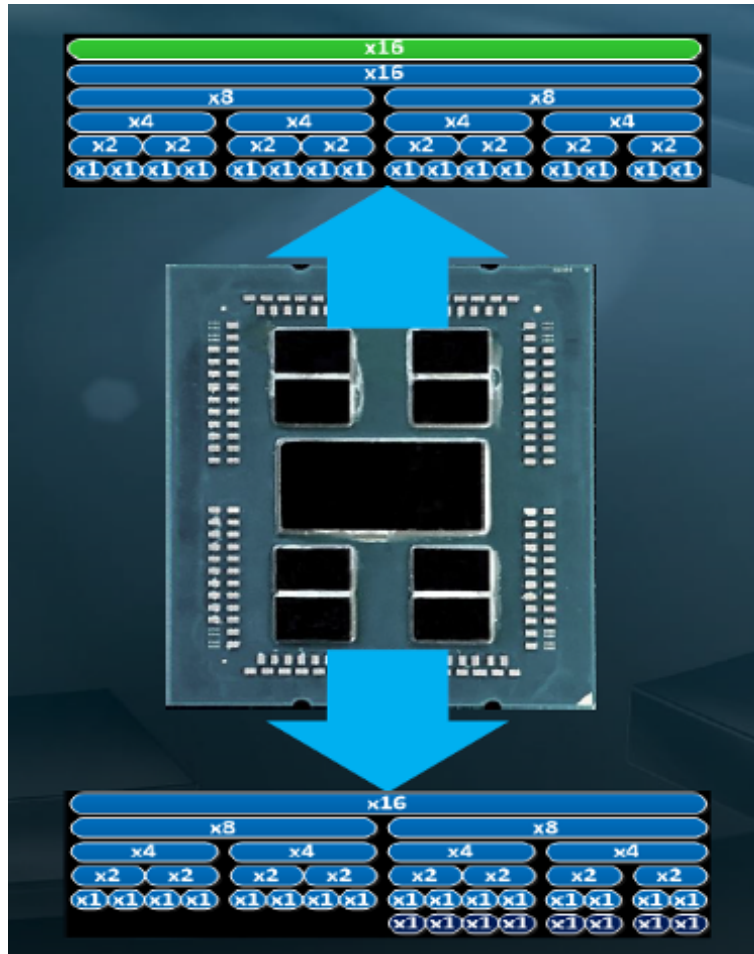
Figure 52. AMD Rome PCIe and how bifurcation can be used: with a x16 PCIe you can split it in multiple ways: 1 x8 and 2x4, or 4x4 [45]
