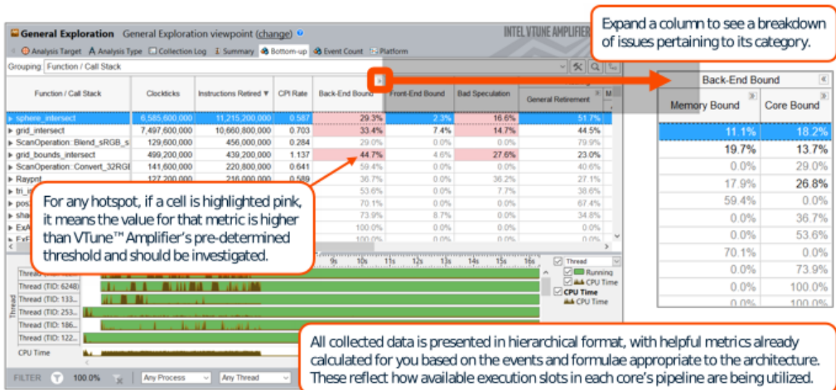
Figure 37. Intel VTune Amplifier (uarch-exploration)
