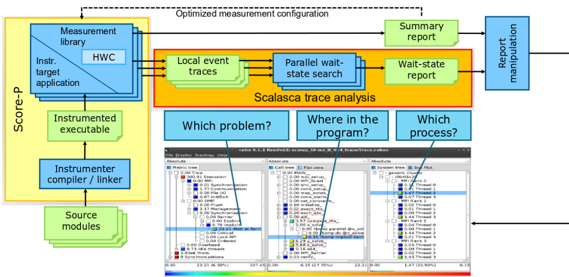
Figure 31. Scalasca workflow
