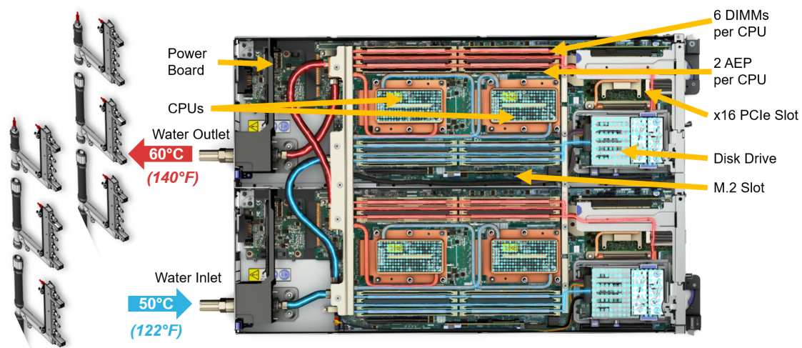
Figure 49. Lenovo ThinkSystem SD650 [105], [106]
