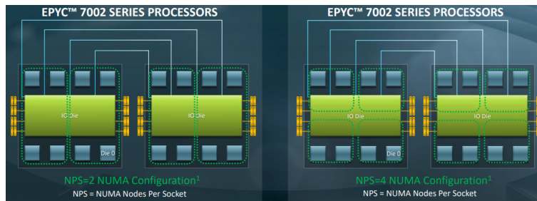
Figure 61. AMD Rome Numa Representations [47]
