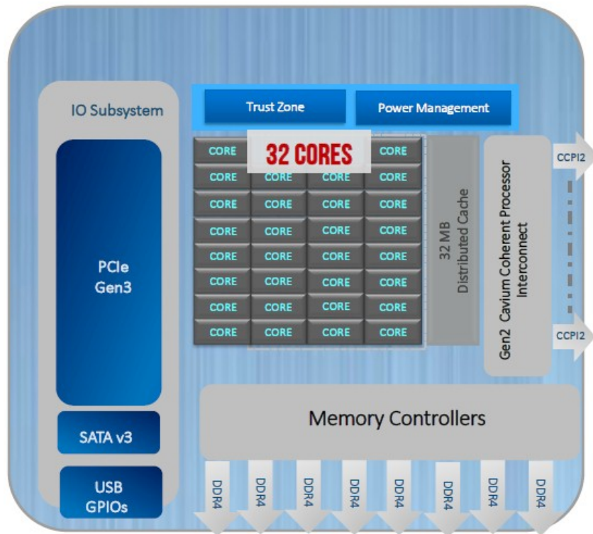
Figure 2. ThunderX2 block diagram [52]
