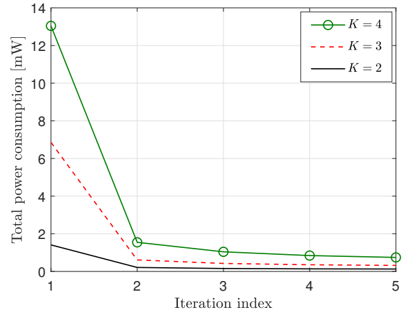
Fig. 2: Transmit power consumption per user [mW].
