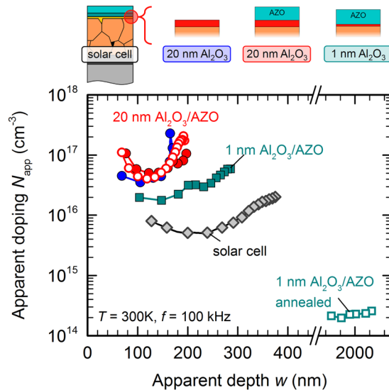
Figure 7. Doping effect by inter-diffusion. Sketch (top) and experimental apparent depth-dependent doping profiles N_{app}(w) determined by CV measurements (bottom) of SLG/Mo/CIGS devices with four different front stacks: a solar cell with standard CdS/i-ZnO/AZO buffer/window stack (grey), 20 nm of \text{Al}_2\text{O}_3 (blue), 20 nm of \text{Al}_2\text{O}_3 covered with AZO (red), and \approx 1 nm of \text{Al}_2\text{O}_3 covered with AZO (green). Open symbols report the dopant concentration after the full device had been annealed for 60 s at 350^\circ\text{C} in nitrogen.
