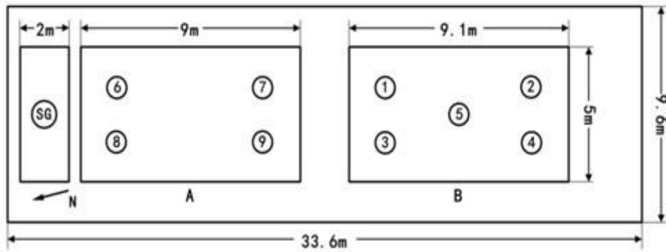
Figure 2. Top: Gravimetric building at Changping Campus of NIM, where the CCM.G-K2.2017 was held. Bottom: Scheme of pillars and sites at the underground comparison station.
