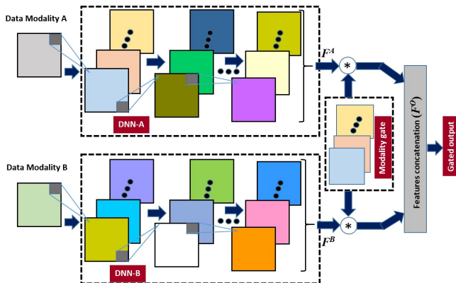
Fig. 1. Proposed data dependent fusion of latent representations, F^A and F^B extracted using DNN-A and DNN-B respectively. A modality gate is used for filtering F^A and F^B to realize improved fusion
