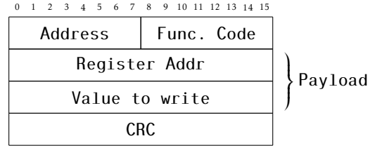
Figure 6. Example of a Modbus frame with a payload containing messages between MTU and RTU.
