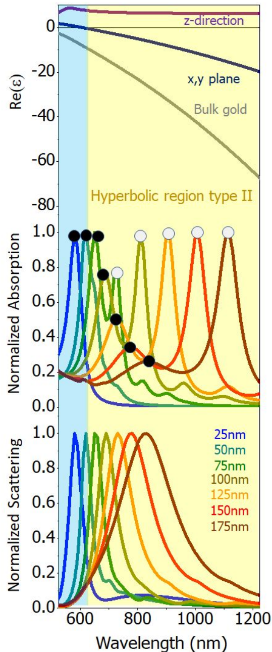
Supplementary Figure S1. Top panel: real part of the dielectric function of a HMM of type II made of multilayers of Au (10 nm each) and of a dielectric material (20 nm each) with n = 1.5 calculated using the effective medium theory (z-direction component – violet curve; x-y plane component – blue curve). The grey line is the real part of the dielectric function of bulk gold.
