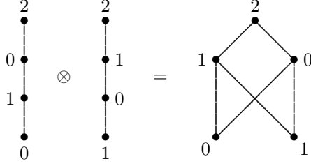
FIGURE 3. The label-matching product of k -lattices is not in general a k -lattice.
