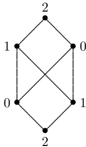
FIGURE 2. The 3-poset representation of a loop.
