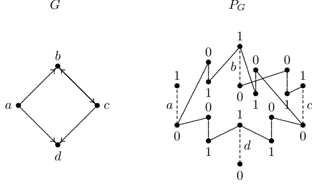
FIGURE 1. Directed graph G and its representation by a 2-poset P_G . Each vertex of G is represented by a two-element chain with label 0 at its bottom and label 1 at its top (dashed lines). Each edge (x, y) of G is represented by a zig-zag from the bottom of the chain representing x to the top of the chain representing y (solid lines).
