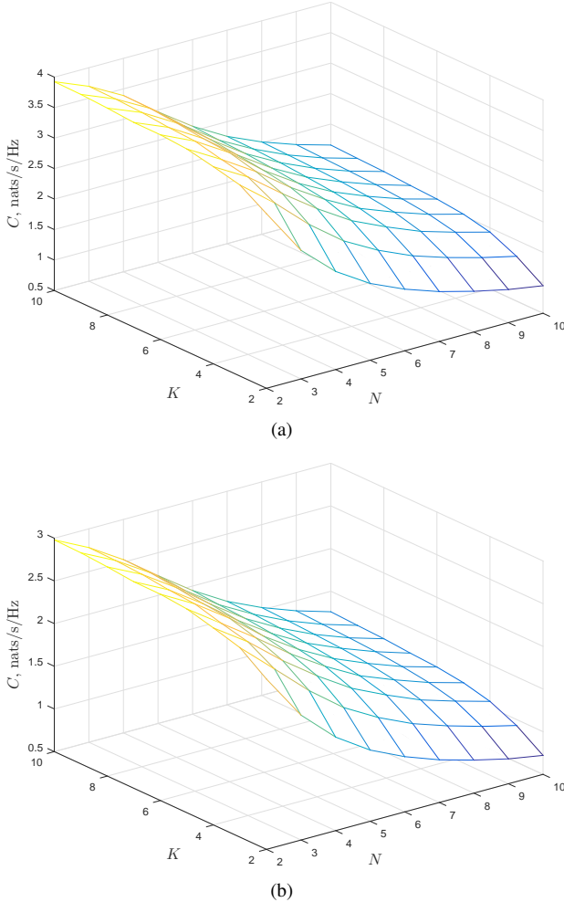
Fig. 3. Per-antenna ergodic capacity versus K and N (a) without imperfections, (b) with imperfections ( \mu = 20 dB, \delta_{t_1} = \delta_{t_2} = \delta_{r_1} = \delta_{r_2} = 0.08 , M = 4 , \alpha = 2\rho )
