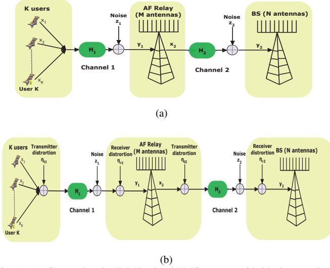
Fig. 1. (a) Conventional AF DH relay MIMO system with ideal transceiver hardware. (b) Generalized AF DH relay MIMO system with residual additive transmitter and receiver hardware impairments.
