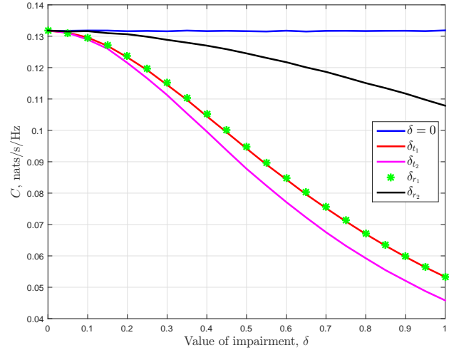
Fig. 10. Per-antenna ergodic capacity versus \delta ( \rho = 5 dB, \beta = 5 , \gamma = 10 , N = 100 , M = 10 , K = 50 , \alpha = 2\rho )
