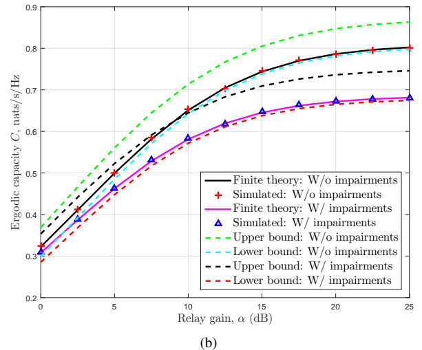
Fig. 2. Per-antenna ergodic capacity versus (a) \rho with and without imperfections ( \delta_{t_1} = \delta_{t_2} = \delta_{r_1} = \delta_{r_2} = 0.08 , K = 2 , M = 4 , N = 3 , \alpha = 2\rho ), (b) \alpha with and without imperfections ( \mu = 15 dB, \delta_{t_1} = \delta_{t_2} = \delta_{r_1} = \delta_{r_2} = 0.08 , K = 2 , M = 1 , N = 4 , \alpha = 2\rho )
