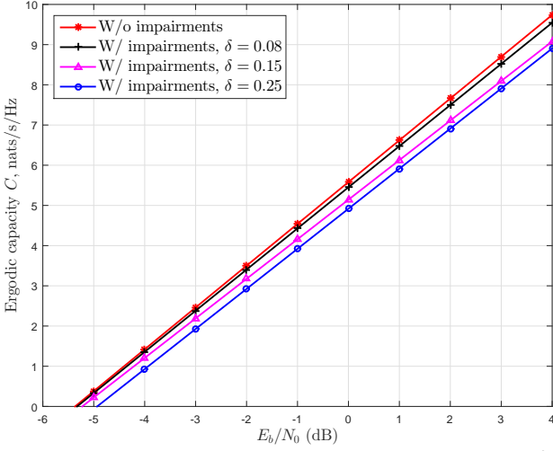
Fig. 5. Per-antenna ergodic capacity with low SNR approximation ( \delta_{t_1} = \delta_{t_2} = \delta_{r_1} = \delta_{r_2} = \delta , K = 2 , M = 3 , N = 2 , \alpha = 2 dB)
