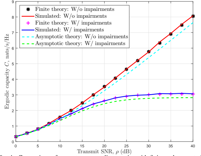
Fig. 4. Comparison of per-antenna ergodic capacity with finite and asymptotic analyses ( \delta_{t_1} = \delta_{t_2} = \delta_{r_1} = \delta_{r_2} = 0.08 , K = 1 , M = 2 , N = 1 , \alpha = 2\rho )
