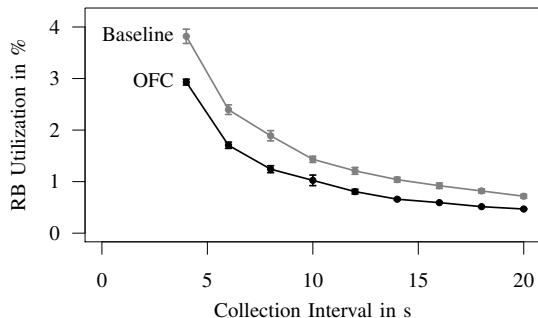
Figure 5. The RB utilization as a function of the collection interval for OFC and Baseline.
