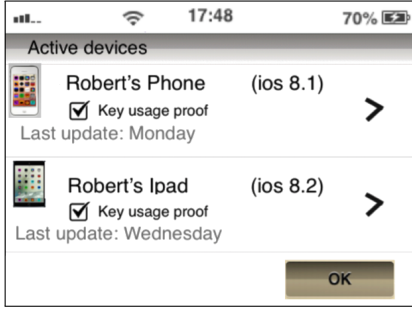
Fig. 3. An example of envisaged GUI that presents the table (D_i, t_i) for i = \{1, 2\} to Robert. The ticked box against the “key usage proof” indicates that the proofs about the usage statement (e.g., last update time) have been cryptographically verified.
