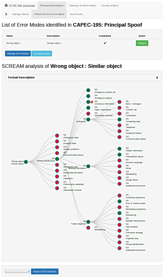
Figure 5: Screen-shot of the retrospectives analysis as performed by using our tool. ‘GA’ are generic antecedent, ‘SA’ specific antecedent. Red antecedent cannot be further expanded, they denote a stop condition in the search for contributors.
