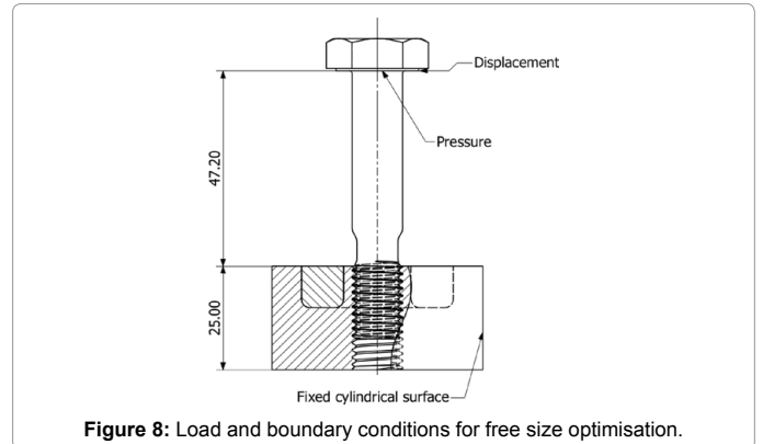
Figure 8: Load and boundary conditions for free size optimisation.
