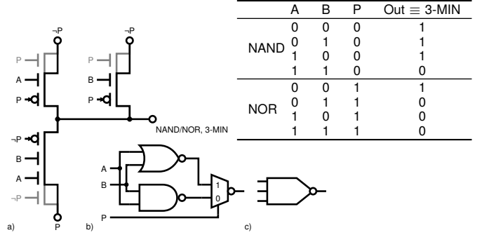
Fig. 2. a) Three-input minority gate as proposed in [11] with optimized series path proposed in [18] and truth table for reference. It uses RFETs, TIGFETs and MIGFETs to show optimization possibilities, black indicates the smallest possible configuration and gray indicates a faster extension; b) Equivalent circuit using CMOS NAND, NOR and MUX gates. c) 3-MIN Circuit symbol.
