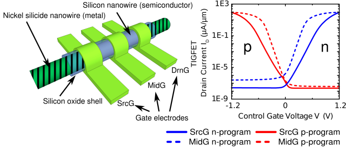
Fig. 1. Silicon nanowire three independent gate FET (TIGFET). The drain gate (DnG) determines channel polarity. The graph shows p-type (red) and n-type (blue) behavior when using the middle gate (MidG) or the source gate (SrcG). Simulated results based on the model used in [14].
