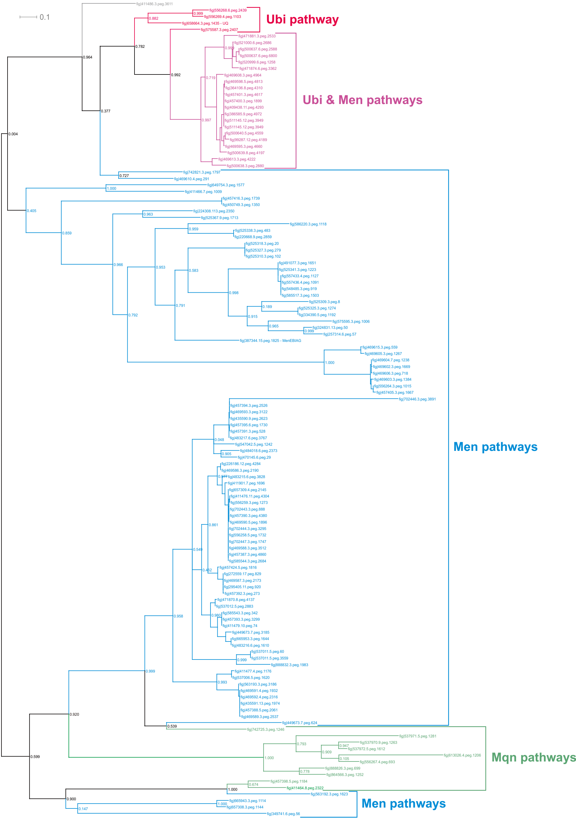
Figure S2. Maximum-likelihood tree for the MenG/UbiE proteins. The co-occurrence of the proteins with quinone biosynthesis pathways is shown by different colours. The SEED identifiers for proteins are shown; for their sequences, see the file Sequences S1 in the Supplementary materials.
