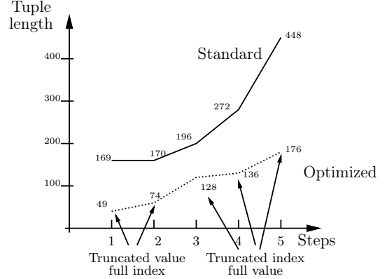
Fig. 3. Tuple length in bits over the steps of Wagner’s algorithm in the basic and the optimized implementations.
