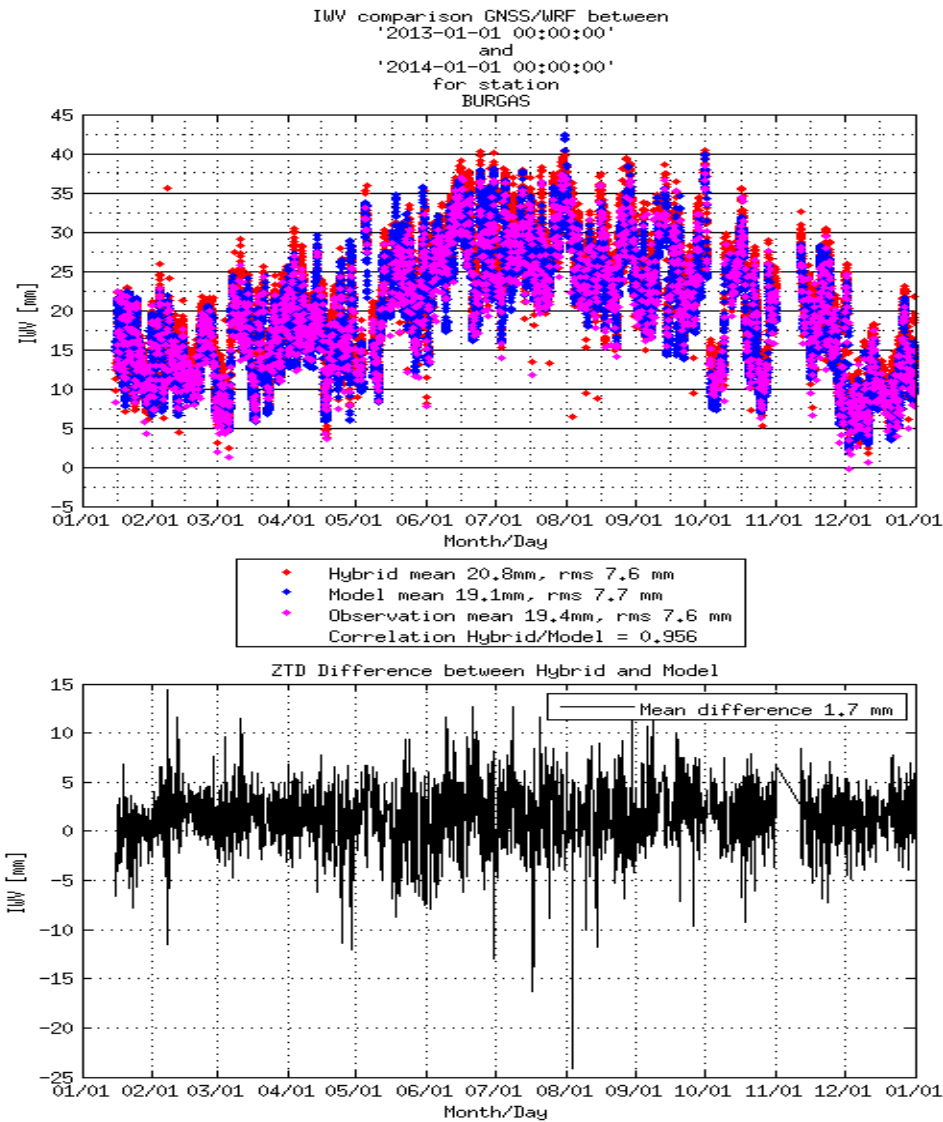
Figure 3: Top figure presents comparison of IwV computations between Hybrid in red, Model in blue and Observation in magenta. The correlation between Hybrid and Model IwVs is 0.956. The bottom figure shows the offset of the Hybrid dataset compared to the Model
