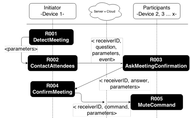
Figure 6. Sequence diagram with the rules activation and the communication process of SilentMeet
