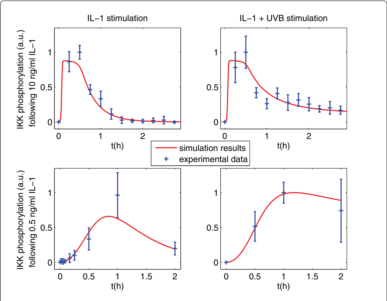
Figure 3 IKKβ phosphorylation following different stimulations - experimental data and simulation results of the model with TRAF extension. Columns show stimulation with IL-1 or IL-1 + UVB (300 J/m 2 ) radiation, respectively, applied at t = 0 s. Rows indicate whether a high (10 ng/ml) or low (0.5 ng/ml) IL-1 dose was applied. A different scaling factor is chosen for the data for 10 and 0.5 ng/ml IL-1 stimulation.
