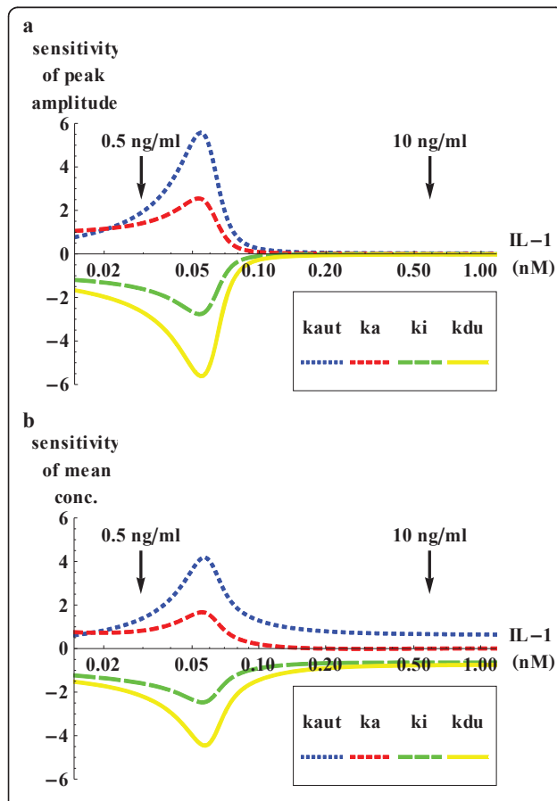
Figure 4 Sensitivity analysis. The relative sensitivity of the (a) peak and (b) mean IKKp concentration to perturbations in the parameters k_a , k_i , k_{aut} , and k_{du} is highly dependent on the IL-1 dose. Sensitivities were calculated and plotted using Mathematica 8.0.
